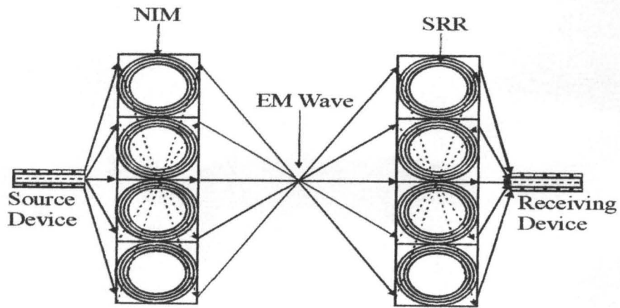
Fig 4.4 Mechanism of WPT Using Negative Index Metamaterial.
