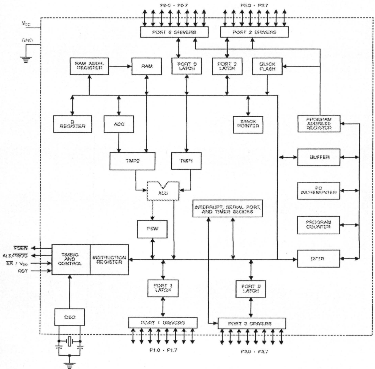
Figs 2.3 Block diagram of AT89C52
