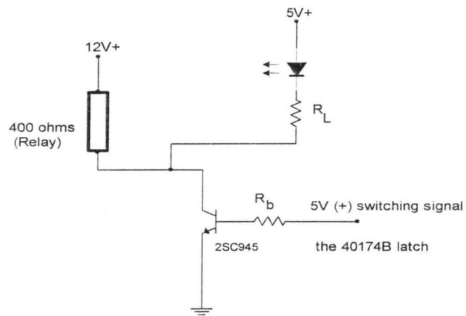
Fig. 3.8 Speed Display
