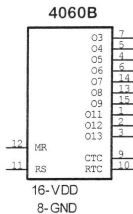
Fig. 2.9 Pin configuration of the 4060B
