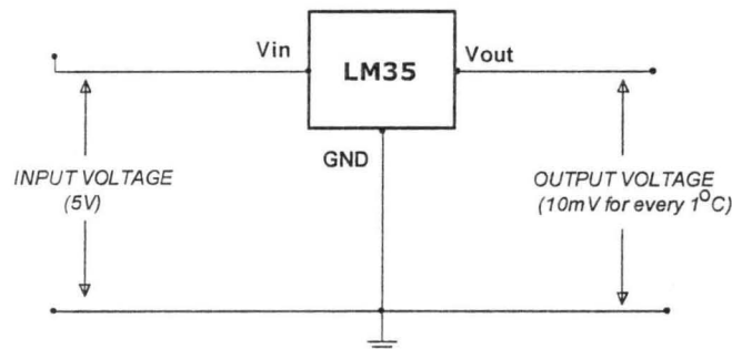
Fig 3.2 Temperature sensor Circuit
