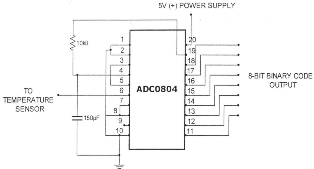
Fig 3.3 The Analogue to Digital Converter circuit
