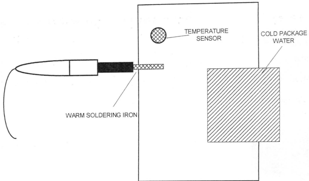
Figure 4.3 Testing Process
