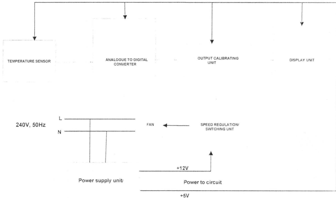
Fig 2.1 The Block Diagram
