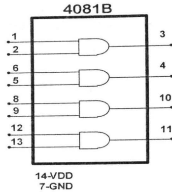
Fig. 2.5 Pin configuration of the 4081B [9]
