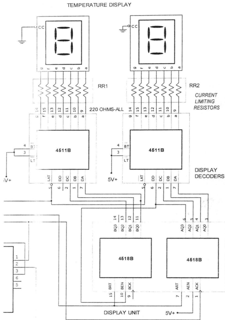
Fig.3.5 Display Unit
