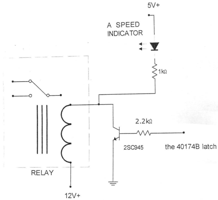
Fig3.7 A single Switching transistor/relay circuit
