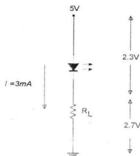
Fig3.9 A single speed indicator Circuit
