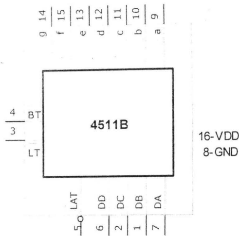
Fig. 2.8 Pin configuration of the 4511B
