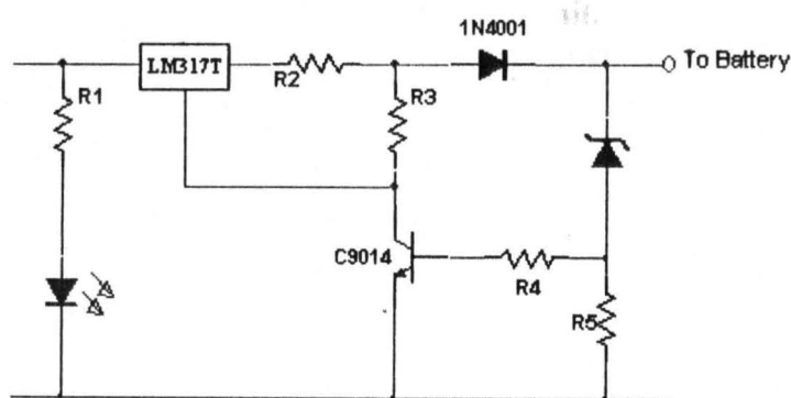
FIG:3 Battery charging unit.
