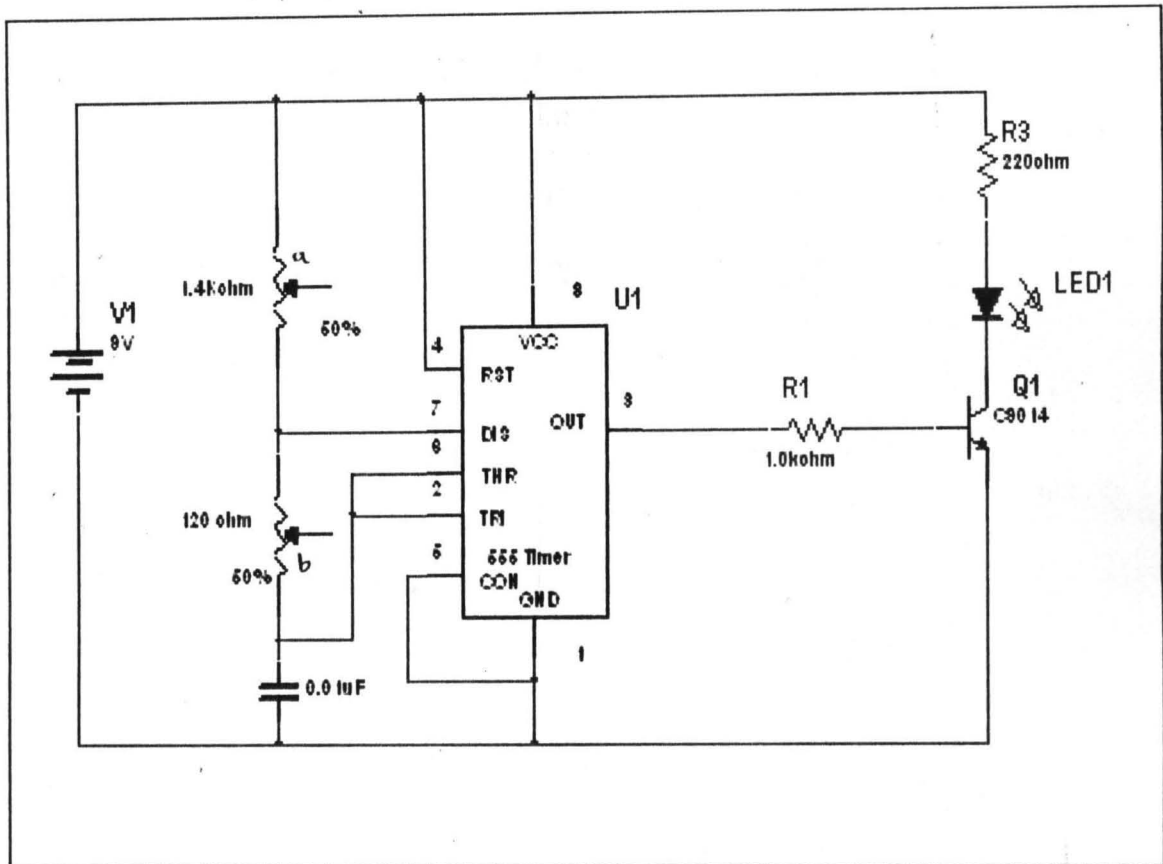
Fig 4: Remote Control Transmitter Circuit
