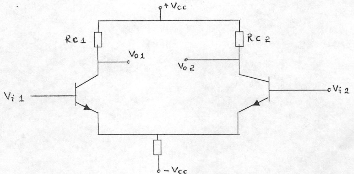
Fig 2.4 Basic differential amplifier circuit.
