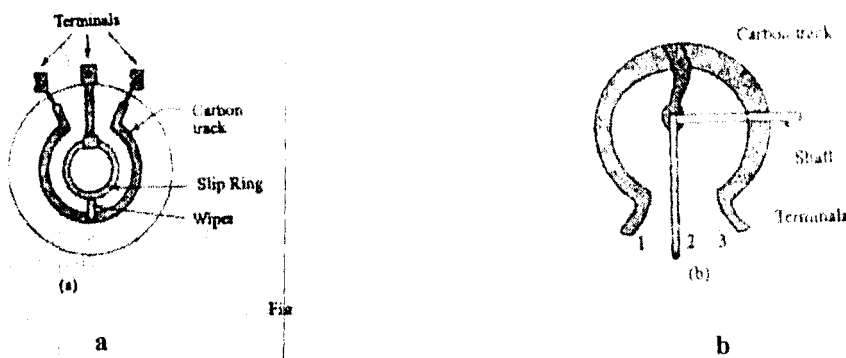
Fig 2.8: form of carbon pots
