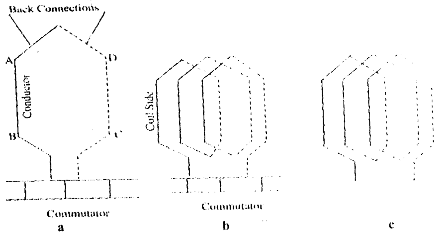
Fig 2.14: conductors
