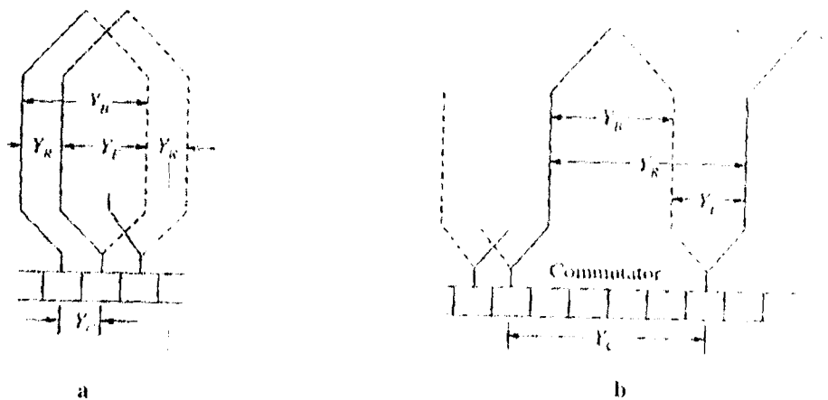
Fig 2.16: shows front and back pitches for lap and wave winding
