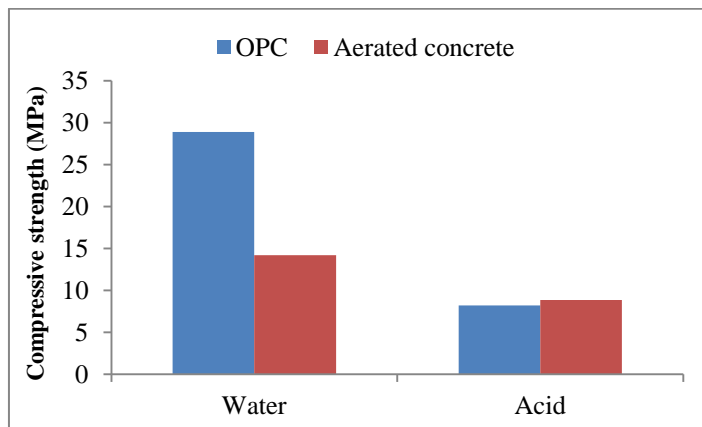
Figure 4: Compressive strength for water cured and acid cured specimens
