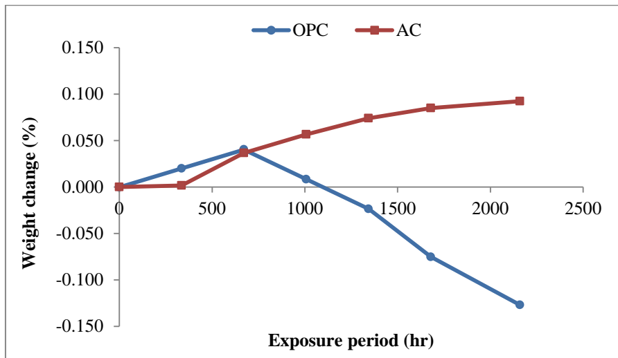
Figure 3: Mass changes in concrete cube specimens
