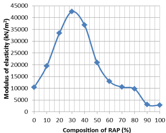
Fig. 12: Variation of modulus of elasticity with varied composition of RAP
