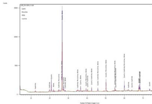
Fig. 3: X-ray Diffraction result for BCS
