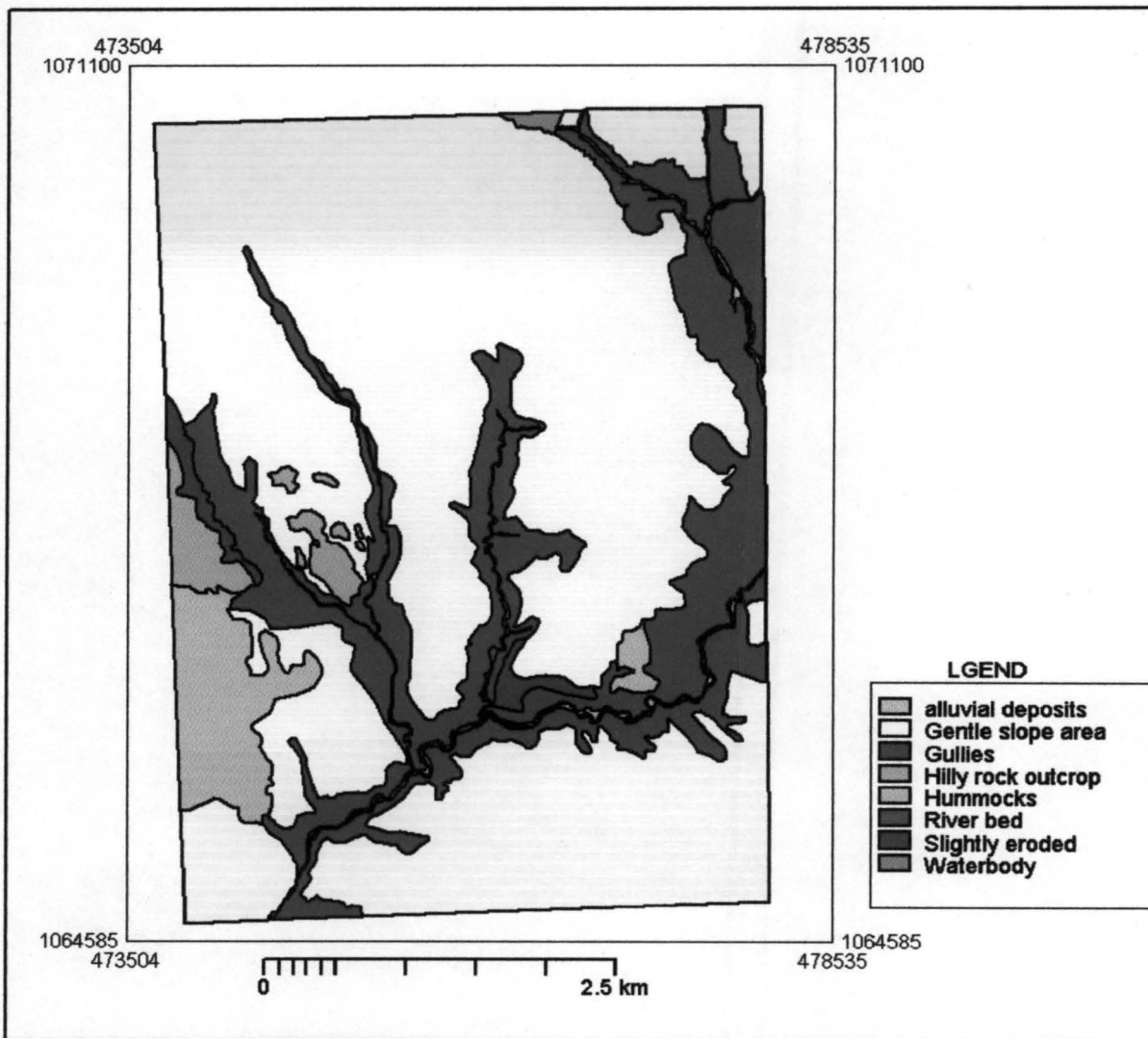
Figure 1.2: Soil map of Farin Lamba
