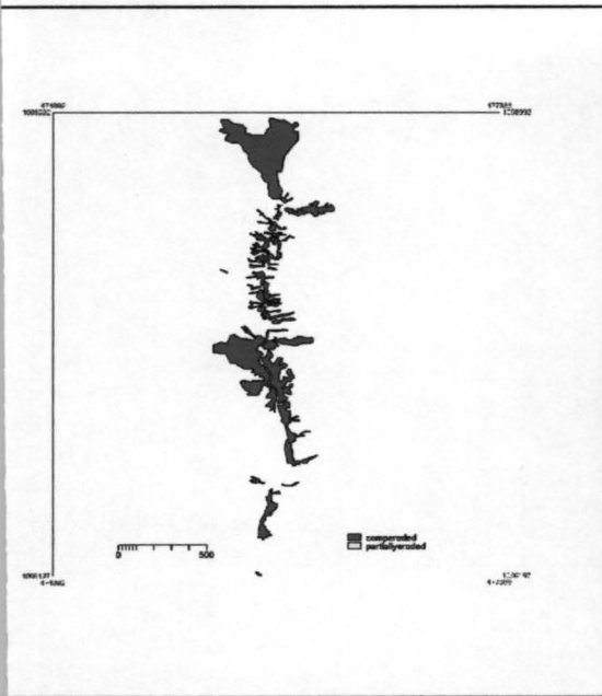
Fig.4.5 Erosion map of catchment B
