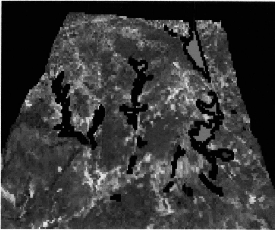
Fig. 4.4: DEM, nature of terrain due to action of erosion
