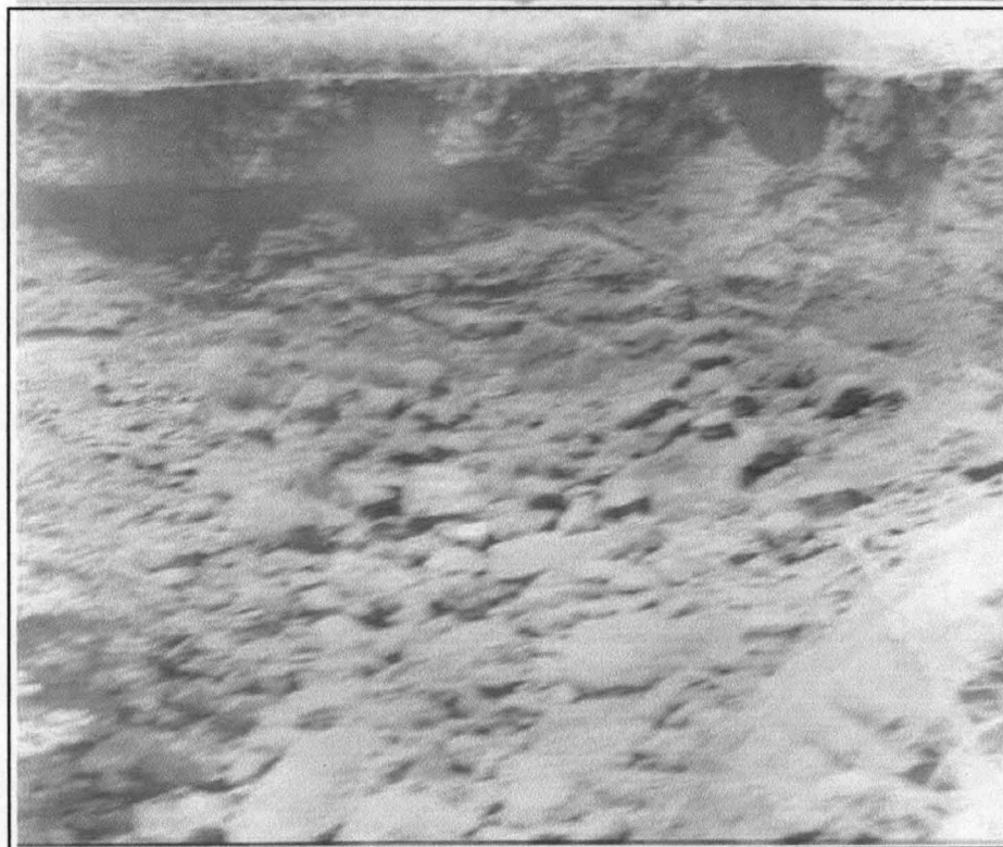
Plate 4.4: Active down cutting and mass movement
