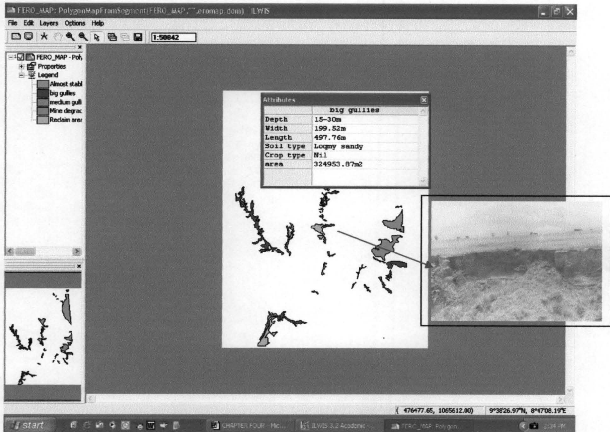
Fig.4.6: GIS Database of the active erosion area
