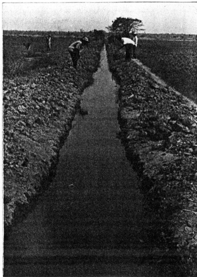
Fig. 6: A field channel being disilted by farmers
