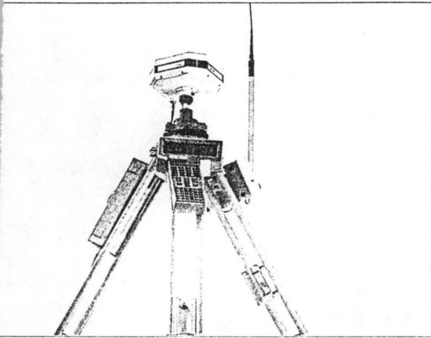
Minimum equipment for real-time reference station.
