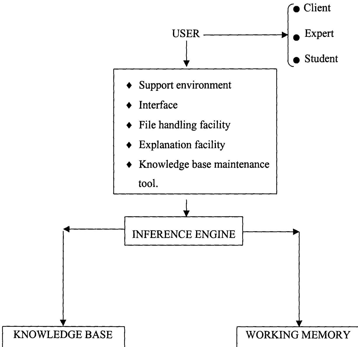
Fig 1. The simple expert system model (After Doukidis et al ).
