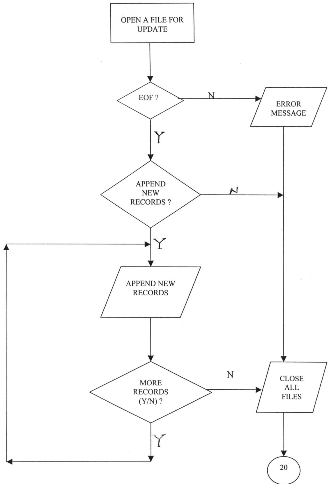
FIG. 5.4 FLOWCHART TO OPEN A FILE FOR UPDATE
