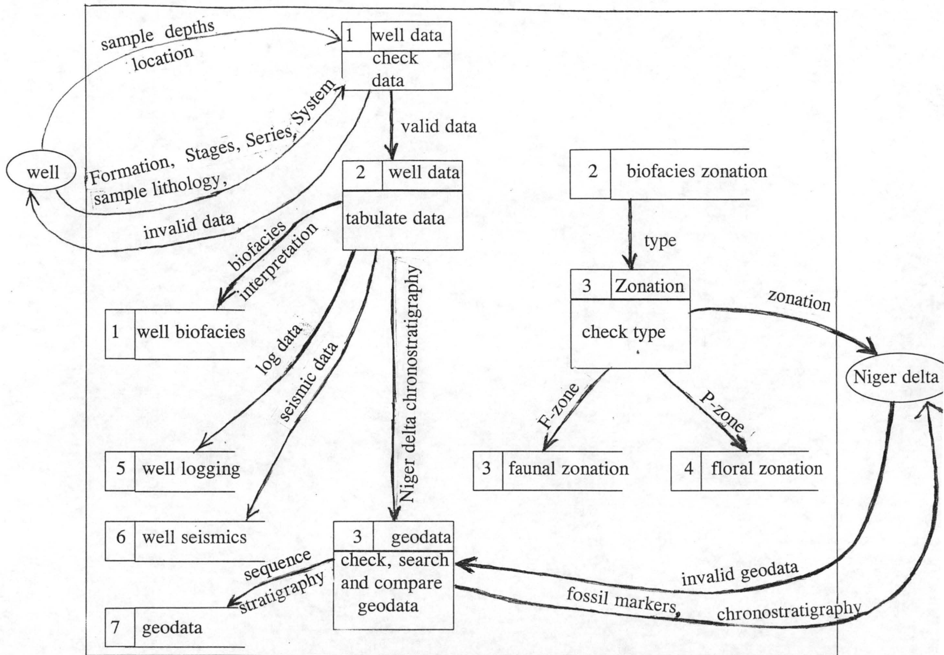
FIG. 3.7 DATA FLOW DIAGRAM OF GEODATA SYSTEM
