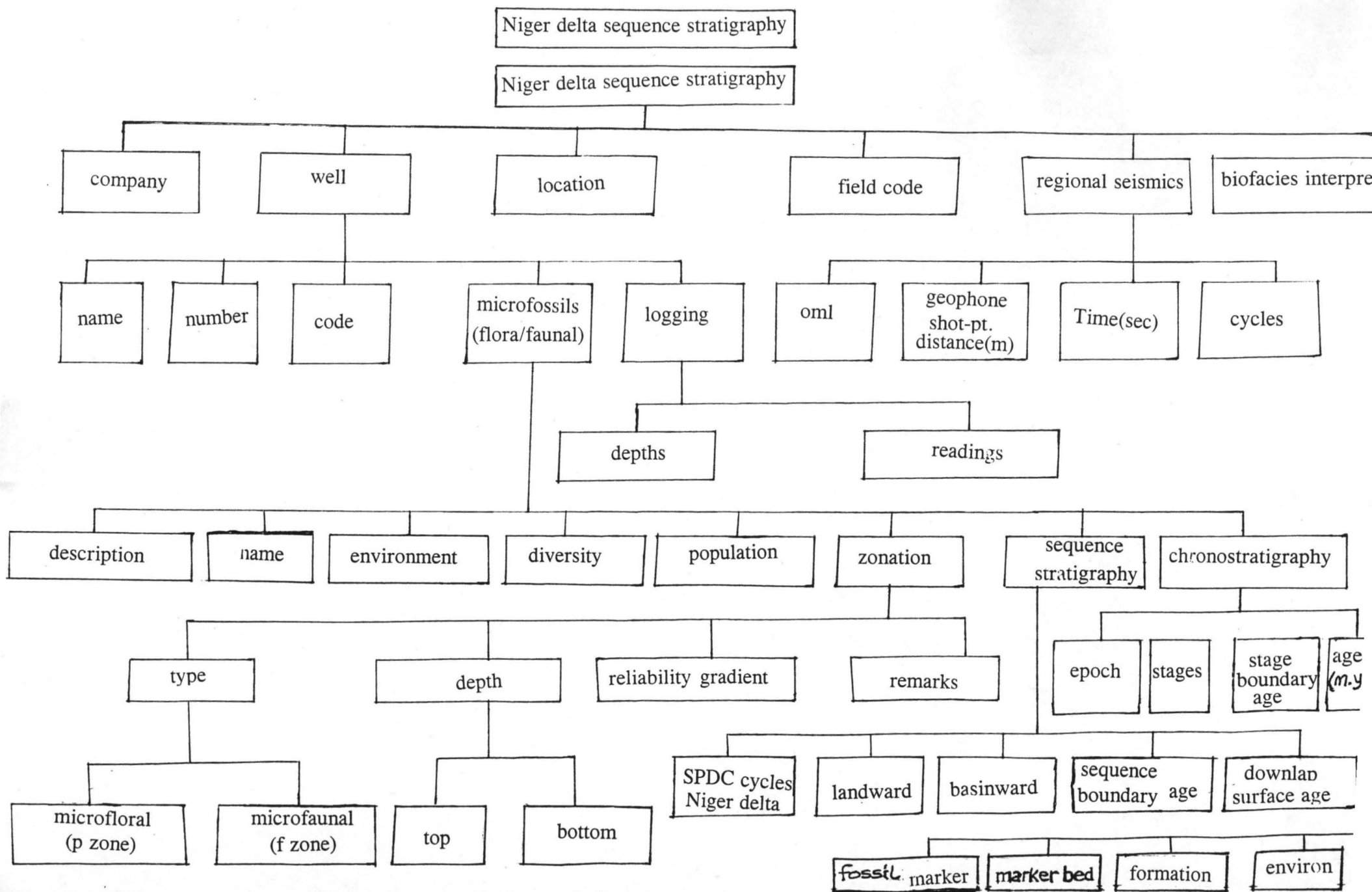
Fig. 5.1 Top down design chart of the Niger delta sequence stratigraphy
