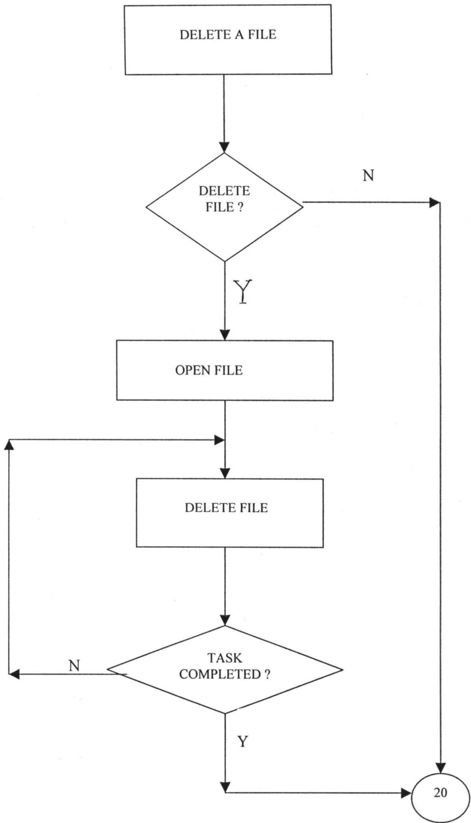
FIG. 5.6 FLOWCHART TO DELETE A FILE
