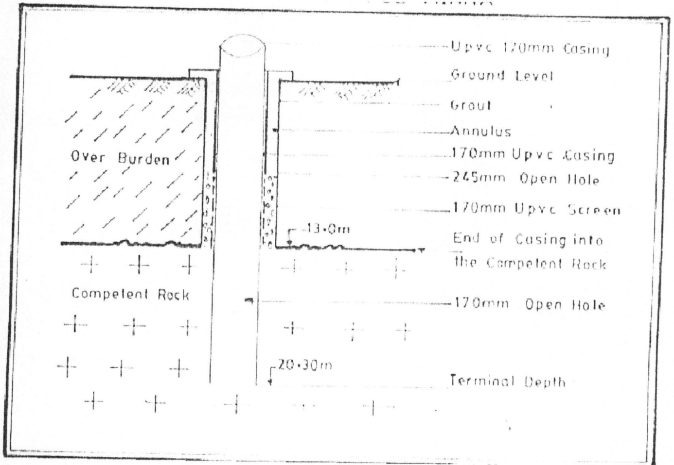
Fig. 2 (a): THE BOREHOLE DESIGN FOR THE BOREHOLE LOCATED z AROUND THE FEMALE HOSTEL (NEAR THE WEATHER STATION) OF F.U.T. BOSSO CAMPUS MINNA.
