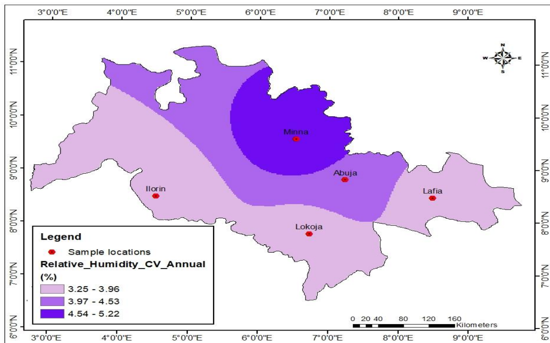
Figure 4.4b. Interpolation of Coefficient of Variation in Annual Relative Humidity
