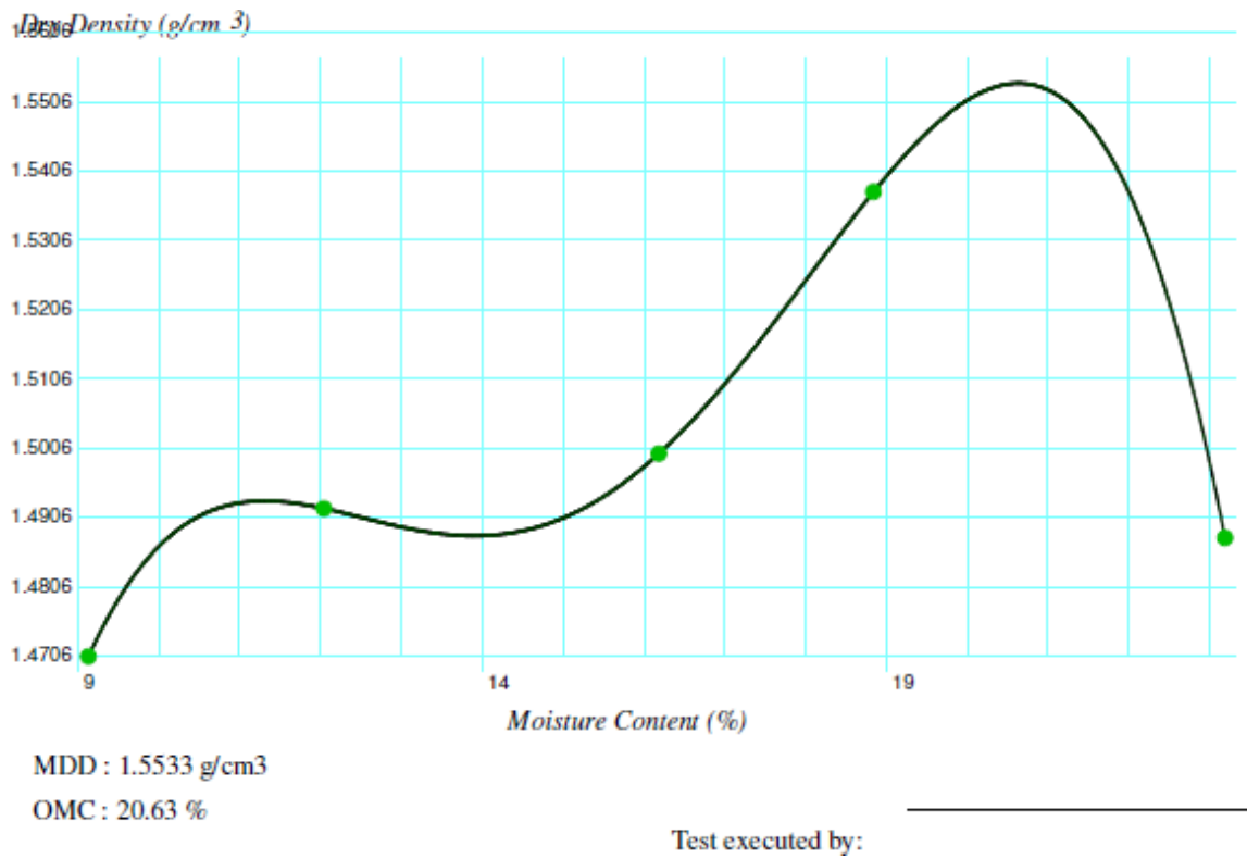
Figure C15: MDD and corresponding OMC of studied soil sample treated with 12% rock flour and 10% lime (BSL)
