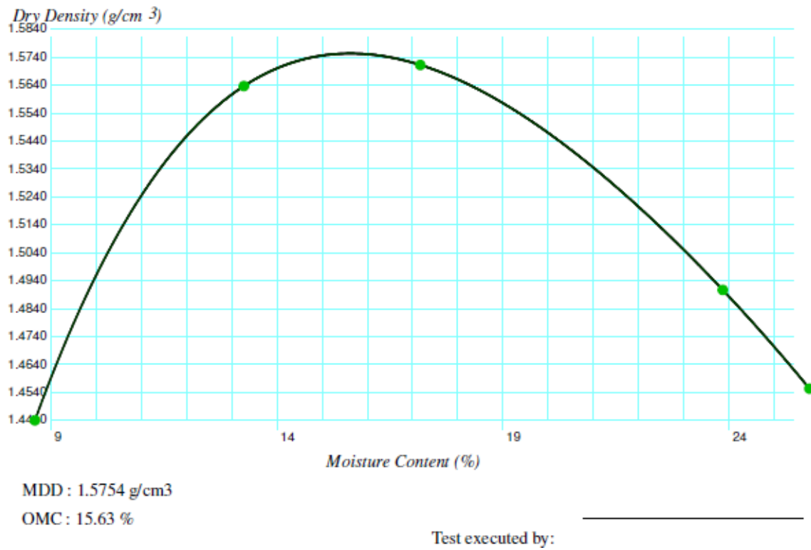
Figure C12: MDD and corresponding OMC of studied soil sample treated with 3% rock flour and 2.5% lime (BSL)
