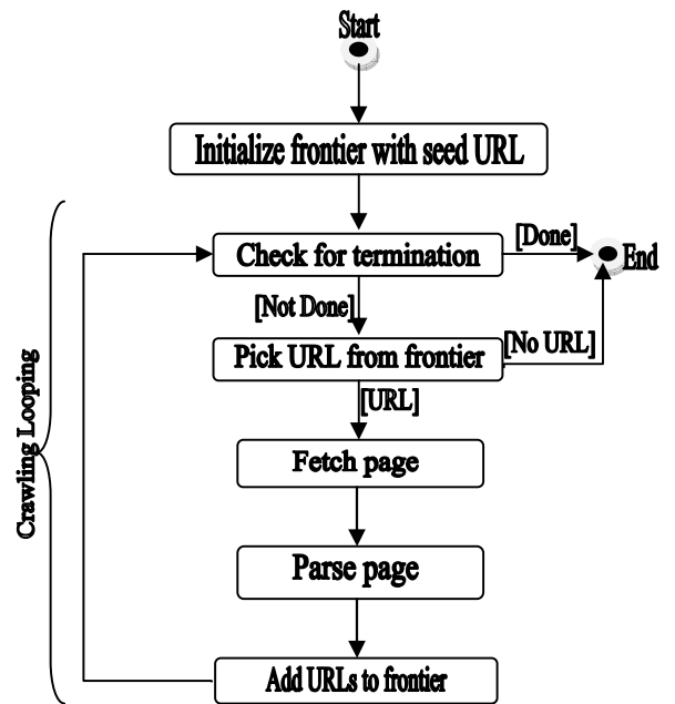
Figure 3. Architecture design of a Crawler
