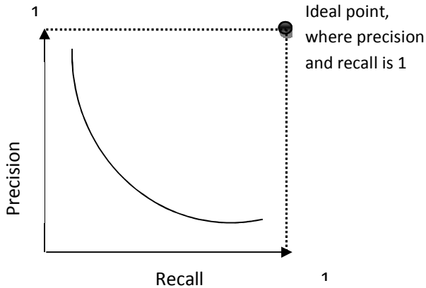
Figure 7. A Typical Recall/Precision Curve
