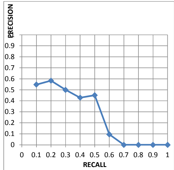
Figure 11. AVERAGE 11-POINT R-P CURVE ACROSS 10 QUERIES ON FEDPOADO WEBSITE RUN FROM THE NEW SYSTEM
