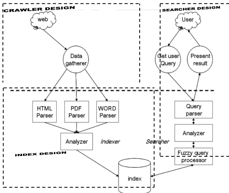
Figure 3. Architecture design of a Crawler
