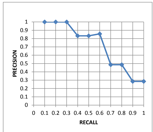
Figure 9. AVERAGE 11-POINT R-P CURVE ACROSS 10 QUERIES ON KP WEBSITE USING LUCENE SEARCH. MEAN AVERAGE PRECISION= 0.7334
