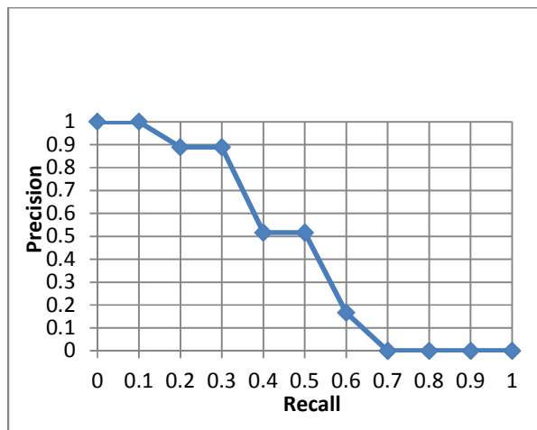
Figure 9. AVERAGE 11-POINT R-P CURVE ACROSS 10 QUERIES ON KP WEBSITE USING LUCENE SEARCH. MEAN AVERAGE PRECISION= 0.7334
