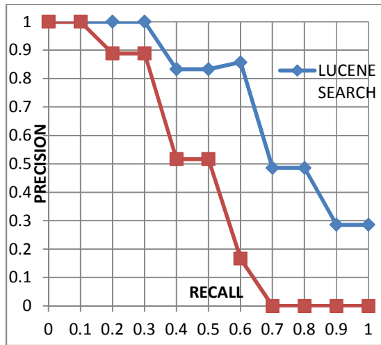
Figure 10. COMPARISON OF 11-POINT AVERAGE OF BOTH SEARCH ENGINE
