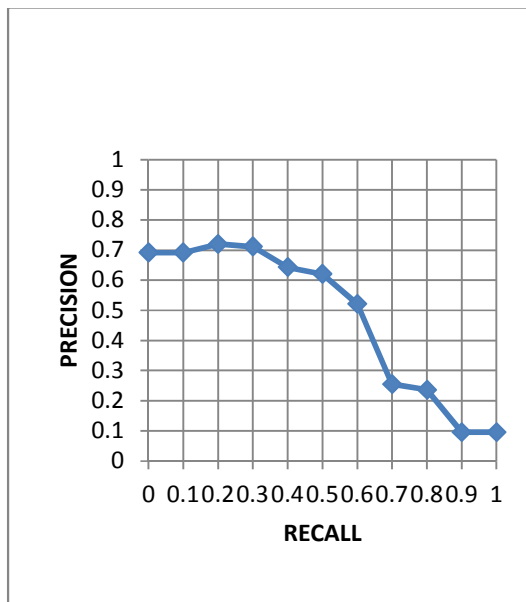
Figure 13. OVERALL R-P CURVE OF THE NEW SEARCH ENGINE MEAN AVERAGE PRECISION = 0.48003
