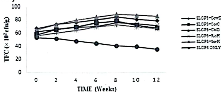
Fig. 3: Total fungi counts (TFC) of spent lubricating oil polluted soil remediated with organic wastes: SLOPS; spent lubricating oil polluted soil, CowD; cow dung, CorC; corn cob, ChiD; chicken droppings, RicH; rice husk, SorH; sorghum husk.
