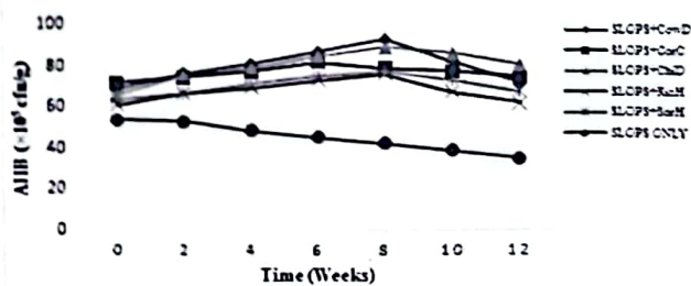
Fig. 1: Aerobic heterotrophic bacterial (AHB) counts of spent lubricating oil polluted soil remediated with organic wastes: SLOPS; spent lubricating oil polluted soil, CowD; cow dung, CorC; corn cob, ChiD; chicken droppings, RicH; rice husk, SorH; sorghum husk.
