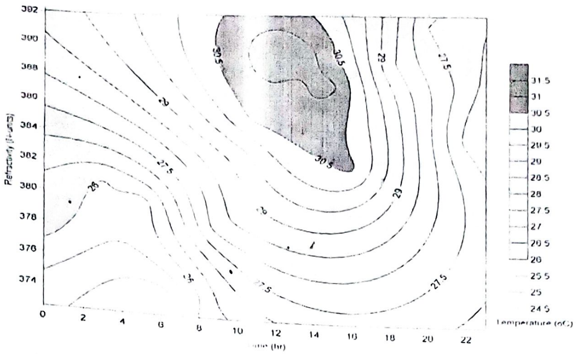
Figure 9: Diurnal Variation of N and T in Dry Season
