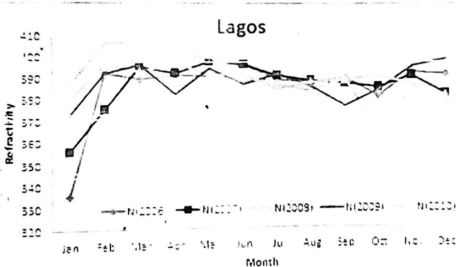
Figure 1: Inter-annual seasonal variation of refractivity
