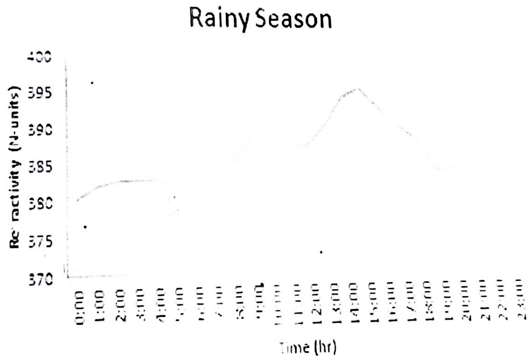
Figure 3: Diurnal Variation of Surface Refractivity
