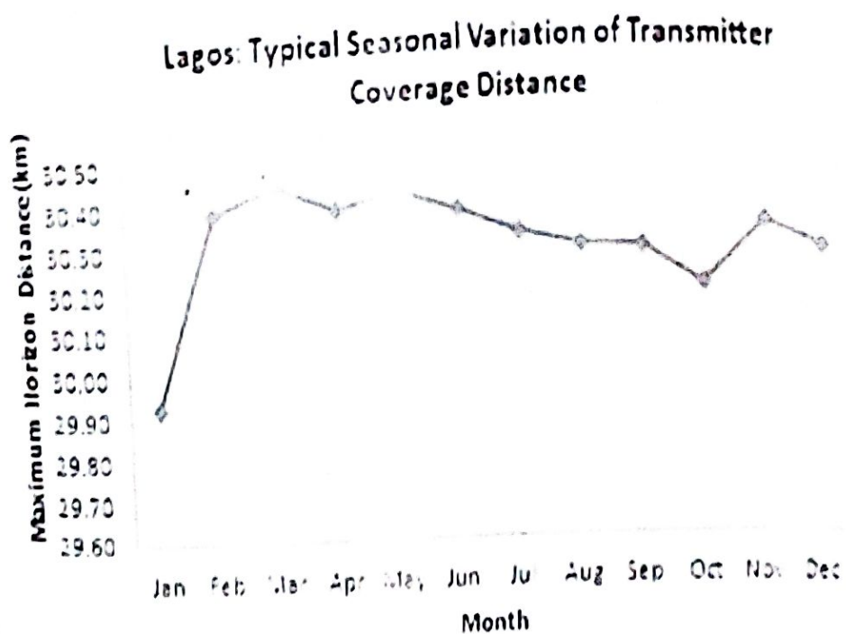
Figure 15: Seasonal Variation of Radio Horizon
