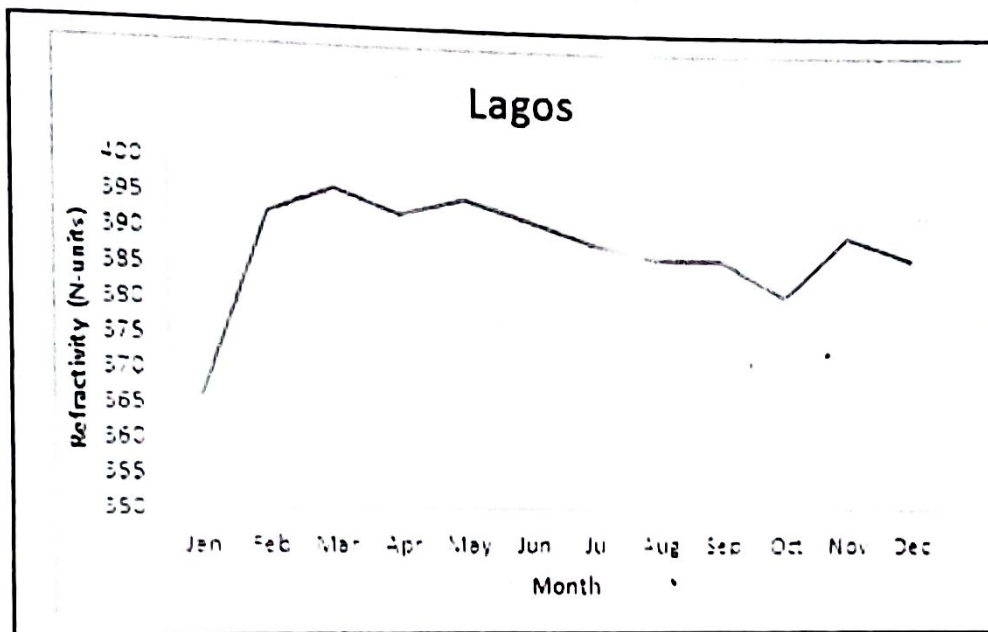
Figure 2: Mean Monthly variation of refractivity
