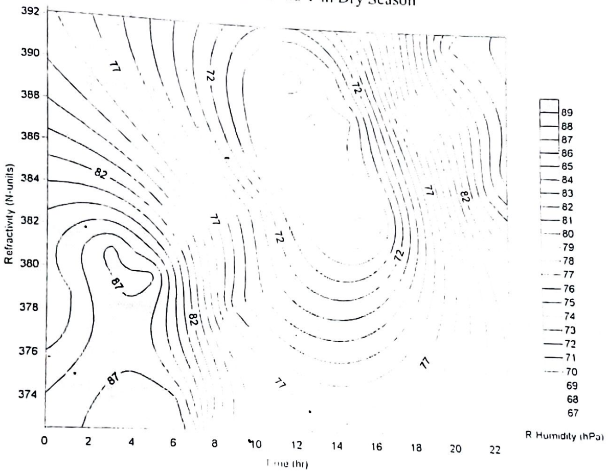
Figure 10: Diurnal Variation of N and H in Dry
