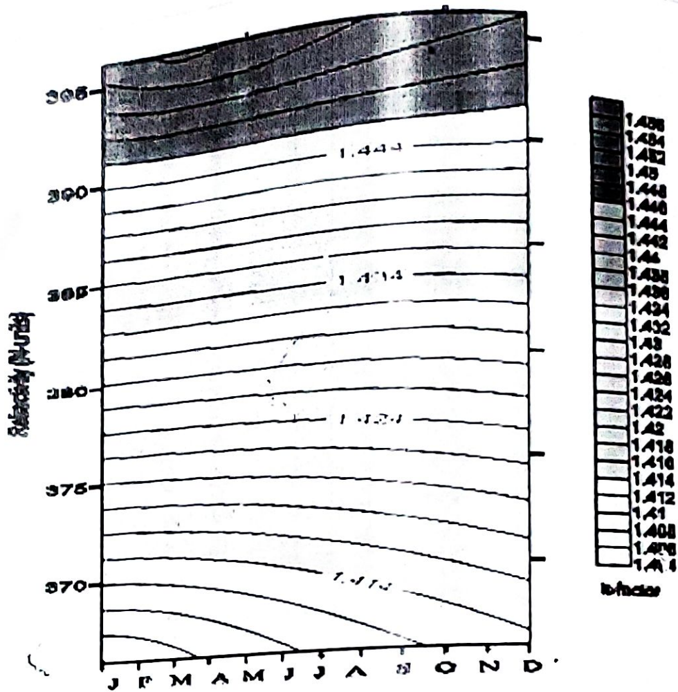
Figure 14: Contour of k-factors Versus N_s
