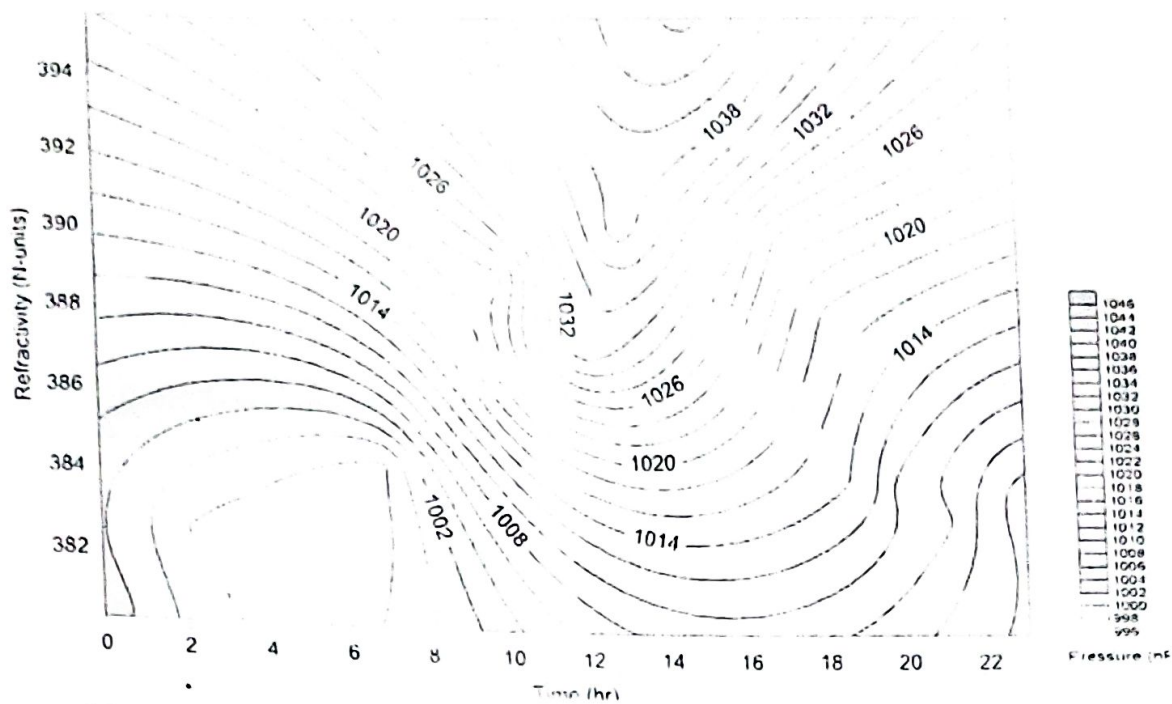
Figure 6: Diurnal Variation of N_s and P in Rainy Season
