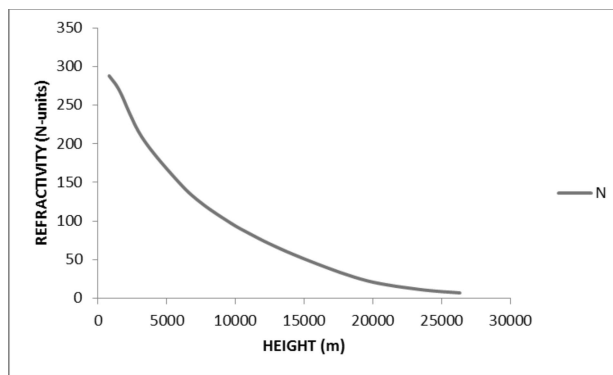
Figure 3: Variation of refractivity with height for January 2014
