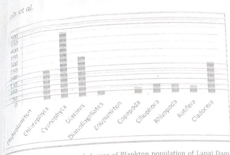
Fig 3: Comparison of classes of Plankton population of Lapai Dam reservoir (The values are mean of three replicates)
