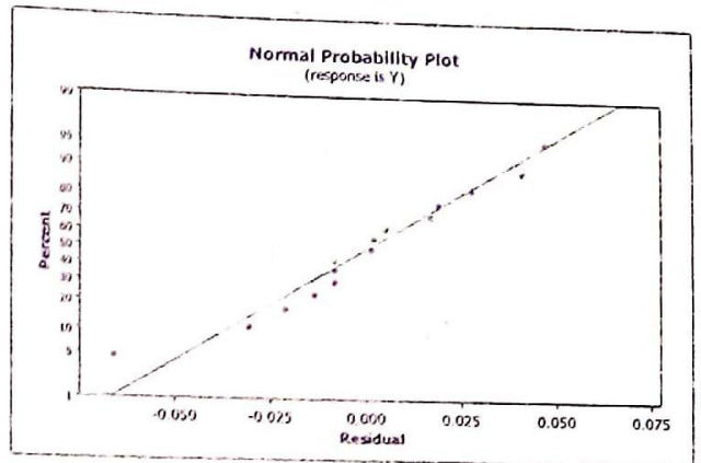
Figure 3: Normal probability plot of residuals for first order tool life data
