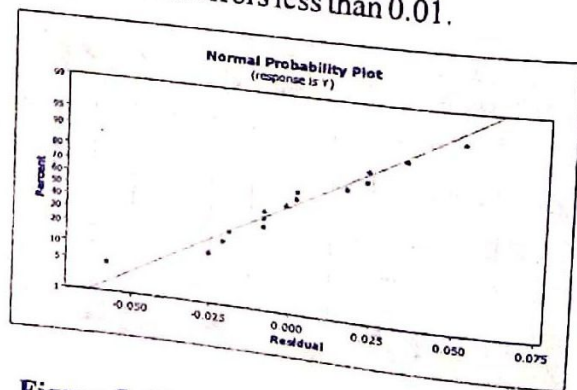
Figure 5: Normal probability plot of residuals for second order tool life data
