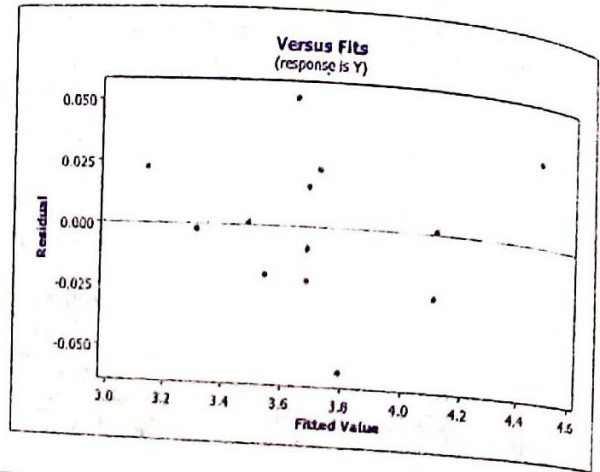
Figure 4: Plot of residual versus predicted response for second order tool life data
