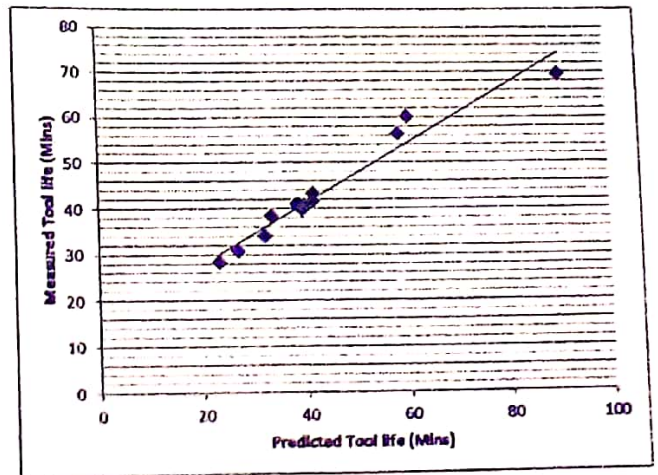
Figure 6: Comparison of measured and predicted tool life
