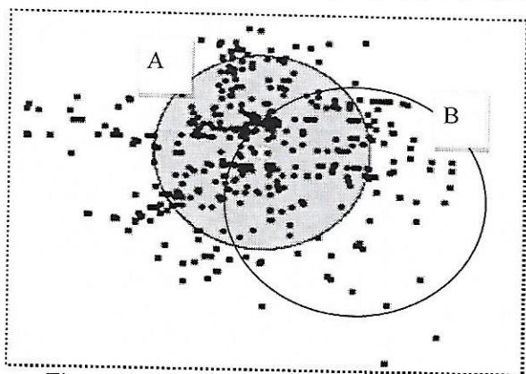
Figure 2. The elements of Standard Distance
