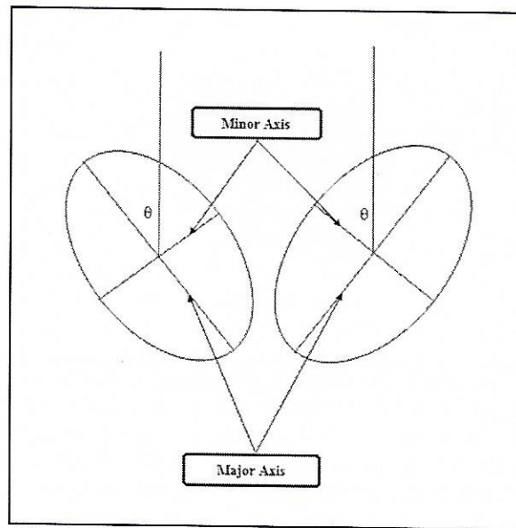
Figure 3. Elements that defines the standard ellipse
