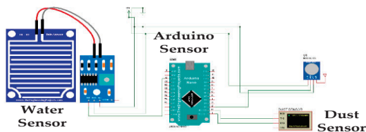
Fig. 3. Circuit diagram of the outdoor unit
