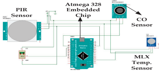
Fig. 2. Simulated circuit diagram of the indoor unit
