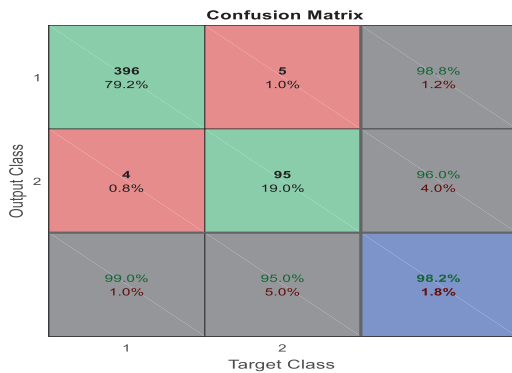
Figure 12. Confusion Matrix for 20 Search Agents and Three Features
