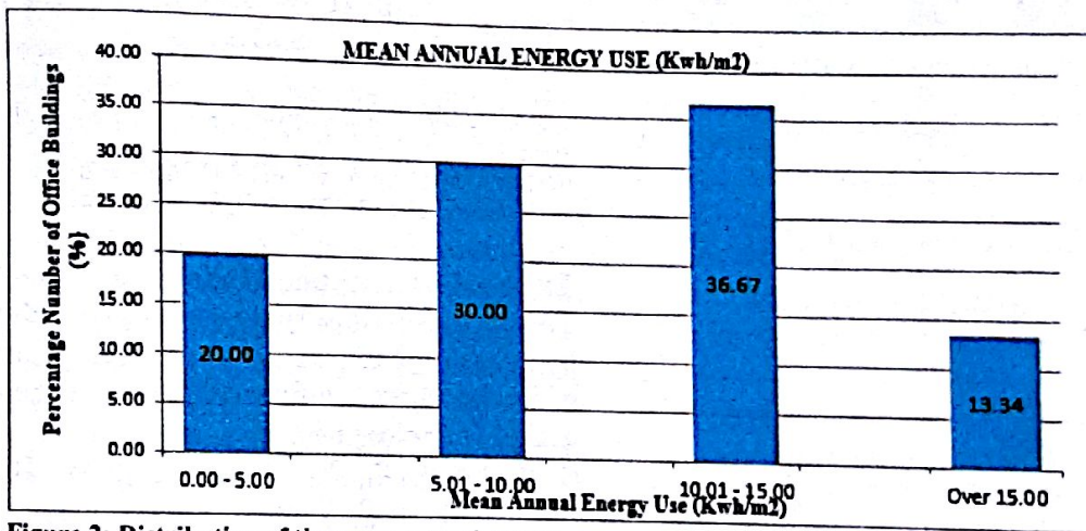
Figure 2: Distribution of the mean annual energy use
