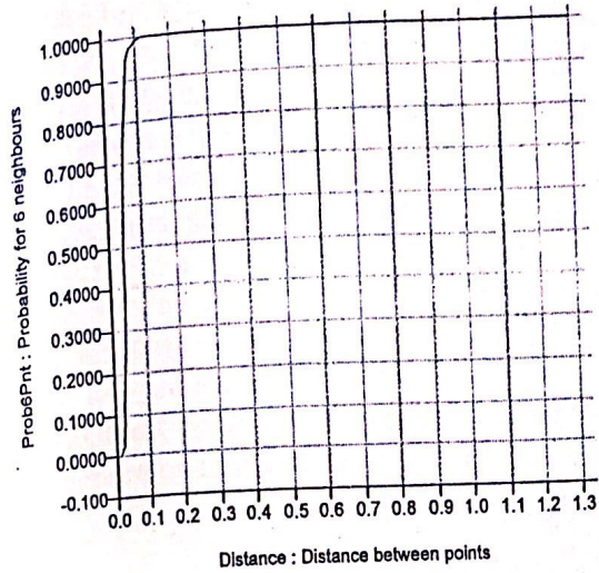
Figure 4: Probability and Distance of Finding Six Neighbours
