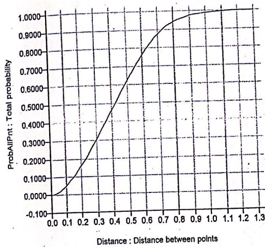
Figure 5: Probability and Distance of Finding Neighbours.
