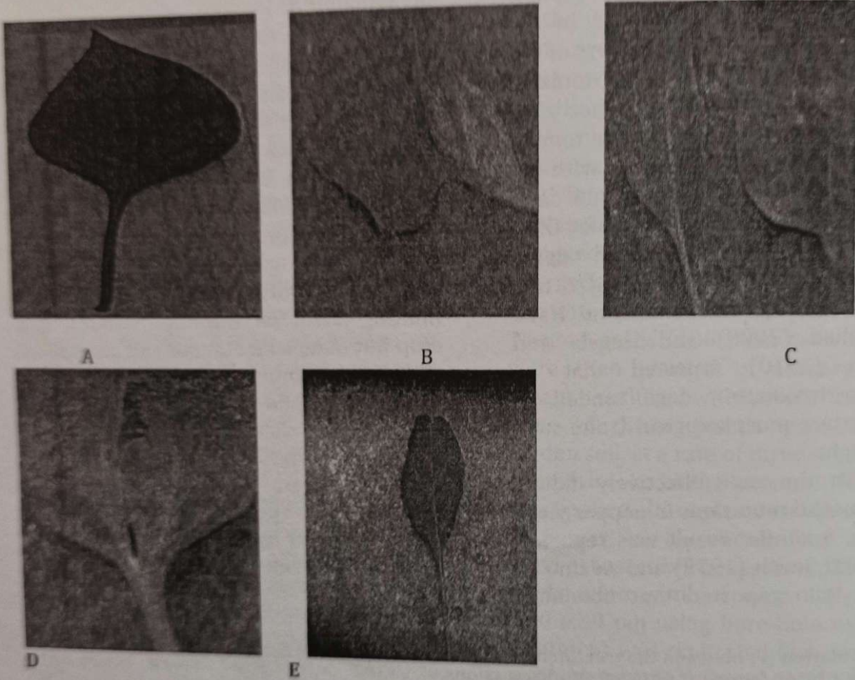
Plate 1: A. Normal leaf of C. annuum var accuminatum B. A leaf with another leafy outgrow at the petiole (90 min IEP) C. Leaves showing invaginated margins (120 min IEP) D. The leaf that turned bifoliage (30 min IEP) E. Leaf with bifurcated apex (60 min IEP).
