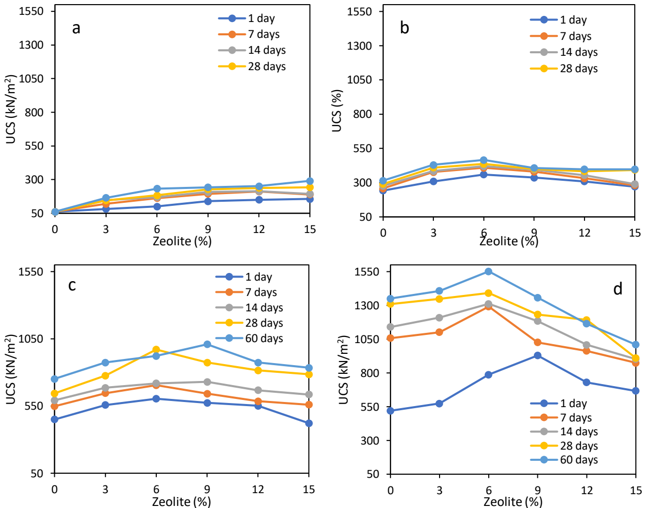
Figure 2. Variation of UCS with varied percent of zeolite at varied curing days for (a) 0% cement, (b) 2% cement, (c) 4% cement (d) 6% cement.
