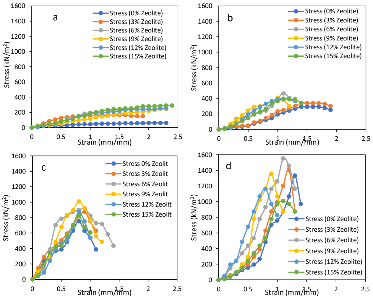
Figure 3. Stress-Strain relation for specimen of varied composition of zeolite for 60 days curing at (a) 0% cement, (b) 2% cement, (c) 4% cement, (d) 6% cement.
