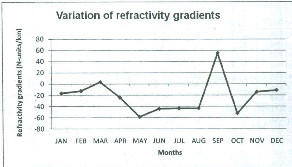
Fig. 5. Seasonal variation of refractivity gradients
