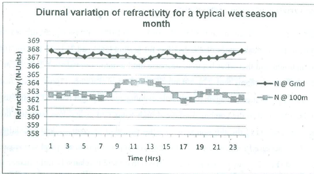
Fig. 2. Mean diurnal variation of N in Minna for a typical wet Season Month
