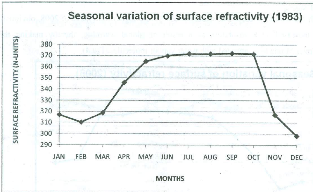
Fig. 4. Seasonal variation of surface refractivity over Minna (1983)
