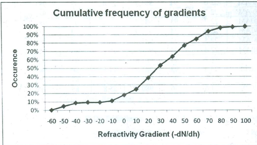
Fig.6. Cumulative frequency of refractivity gradients
