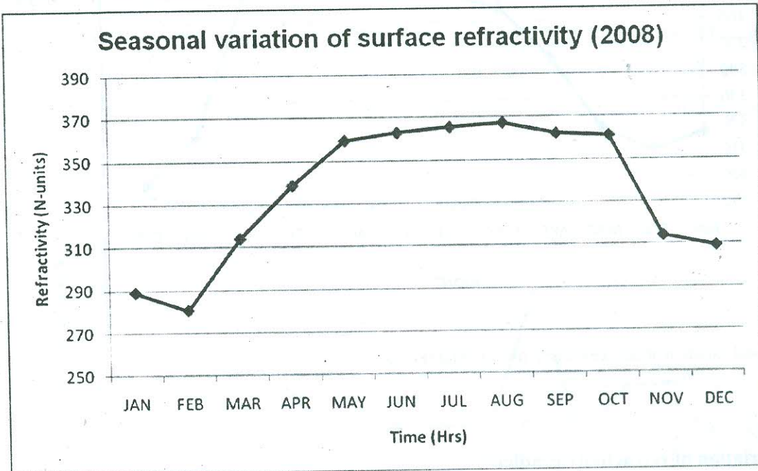
Fig. 3. Seasonal variation of surface refractivity over Minna (2008)
