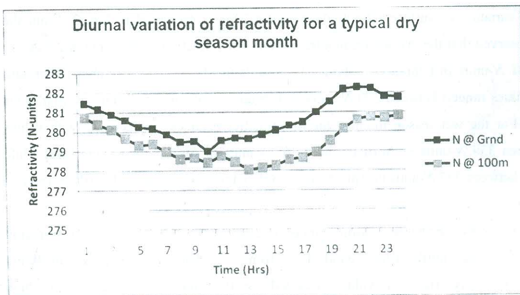
Fig. 1. Mean diurnal variation of N in Minna for a typical dry season month
