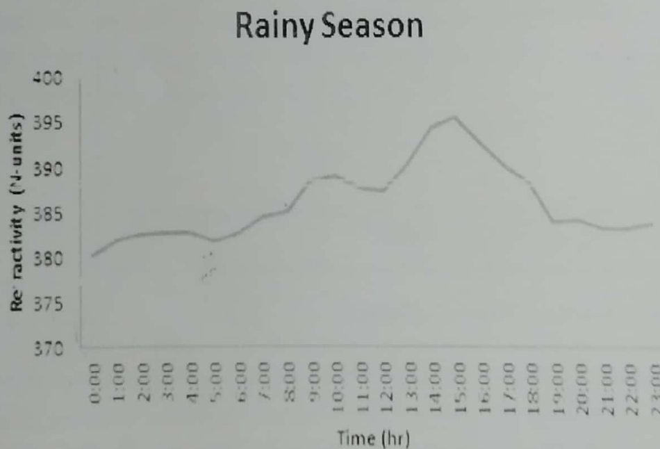
Figure 3: Diurnal Variation of Surface Refractivity
