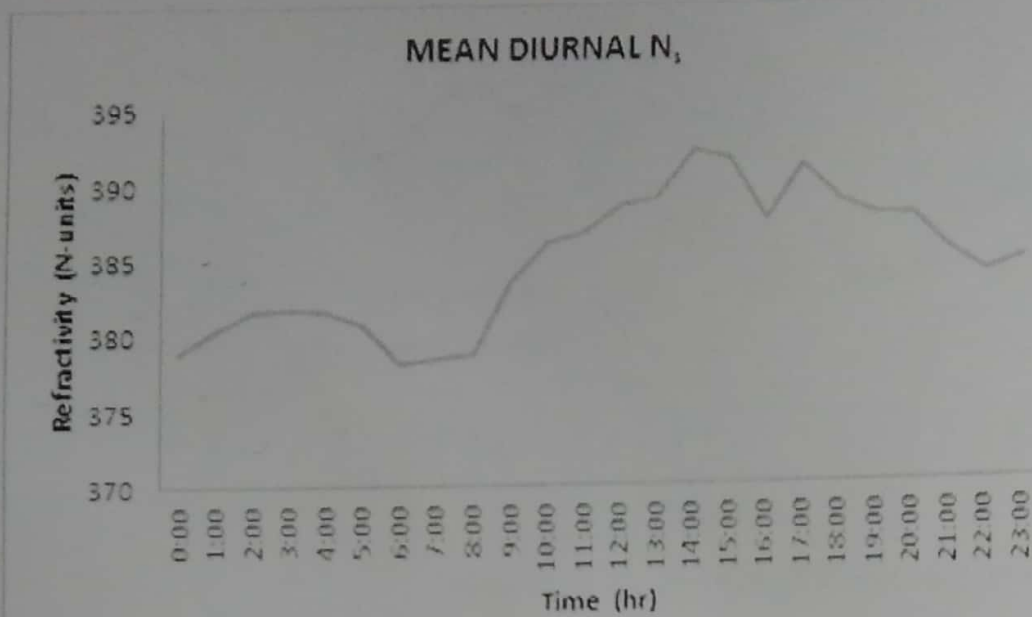
Figure 12: Mean Diurnal Variation of N_s
