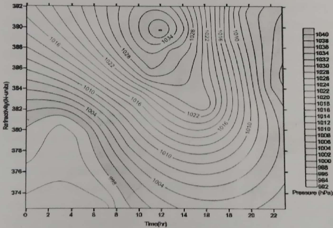
Figure 8: Diurnal Variation of N_s and P in Dry Season
