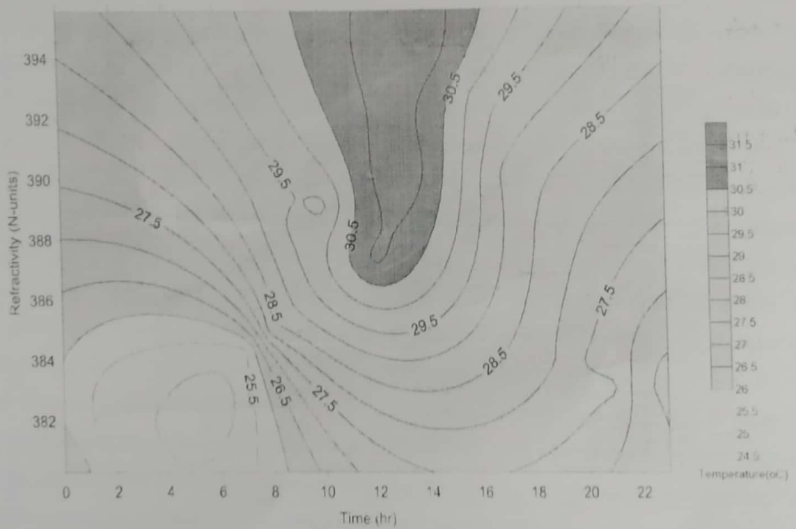
Figure 5: Diurnal Variation of N_e and T in Rainy Season
