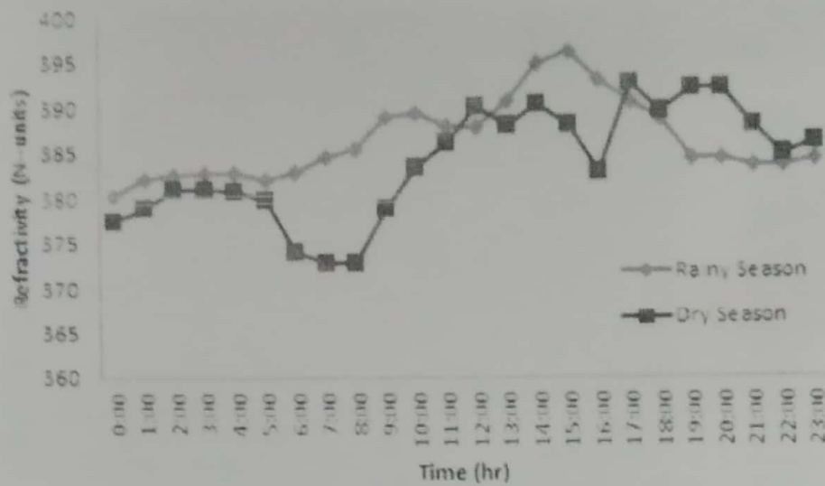
Figure 11: Diurnal Variation of N_s in Rainy and Dry Season
