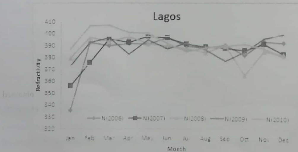
Figure 1: Inter-annual seasonal variation of refractivity
