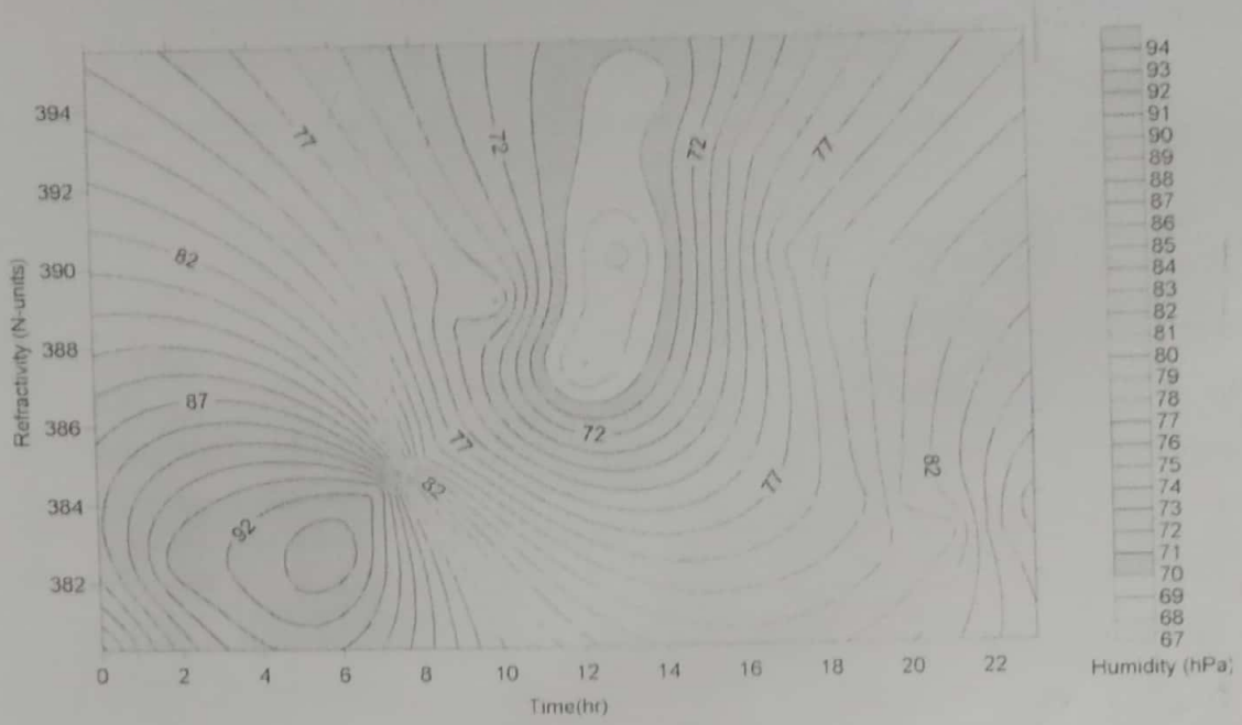
Figure 4: Diurnal Variation of N_e and H in Rainy Season
