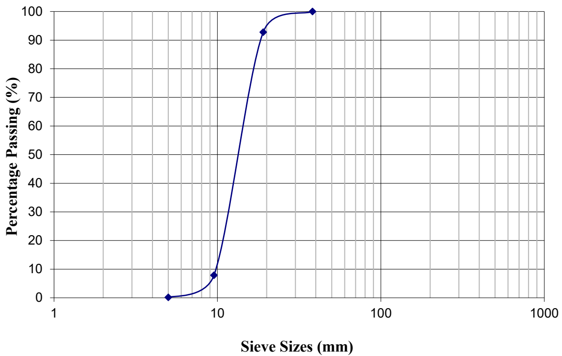
Figure 1: Particle Sizes Distribution of Coconut Shells
