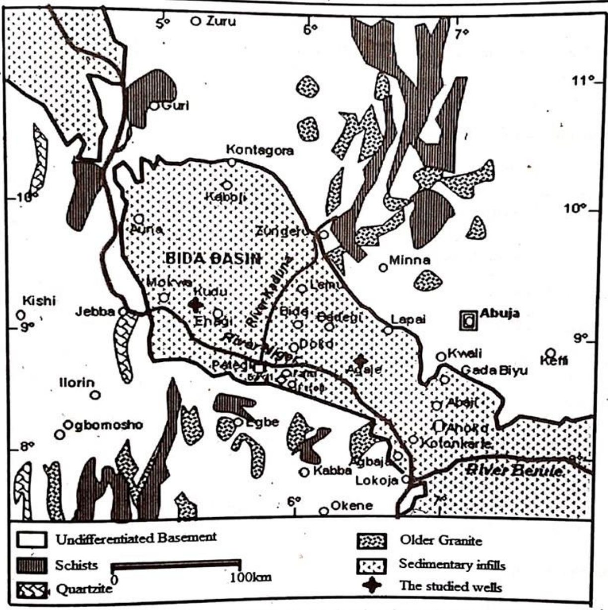
Figure 2: Geology and location of the Bida Basin showing the studied wells (Modified after Obajeet et al. , 2011).
