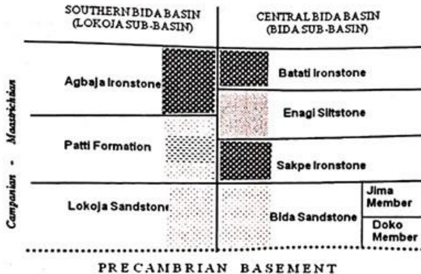
Figure 3: Stratigraphic succession of the Bida basin (After Obajeet al. , 2011).
