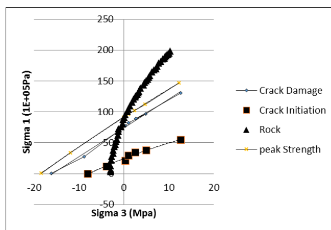
Fig. 7. Rock strength Rock Strength, Crack Initiation, Crack Damage and Peak Strength at 20MPa Confined Pressure for Ughelli sandstone under tri-axial compression
