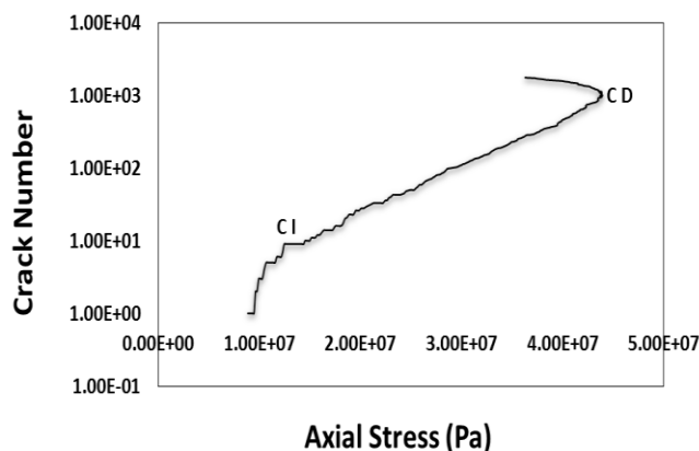
Fig. 3. Crack Initiation (CI) and crack damage (CD) stresses for unconfined axial stress application. The crack number are limited to (1 \times 10^4) particles used for building sandstone sample in the Discrete Element Modelling (DEM).
