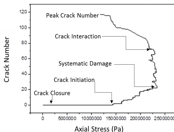
Fig. 6. Crack number and corresponding crack interaction stages: the mechanism of micro-fracturing of Ughelli sandstone at 5 stages for ( \times 10^4 ) particles used for simulation
