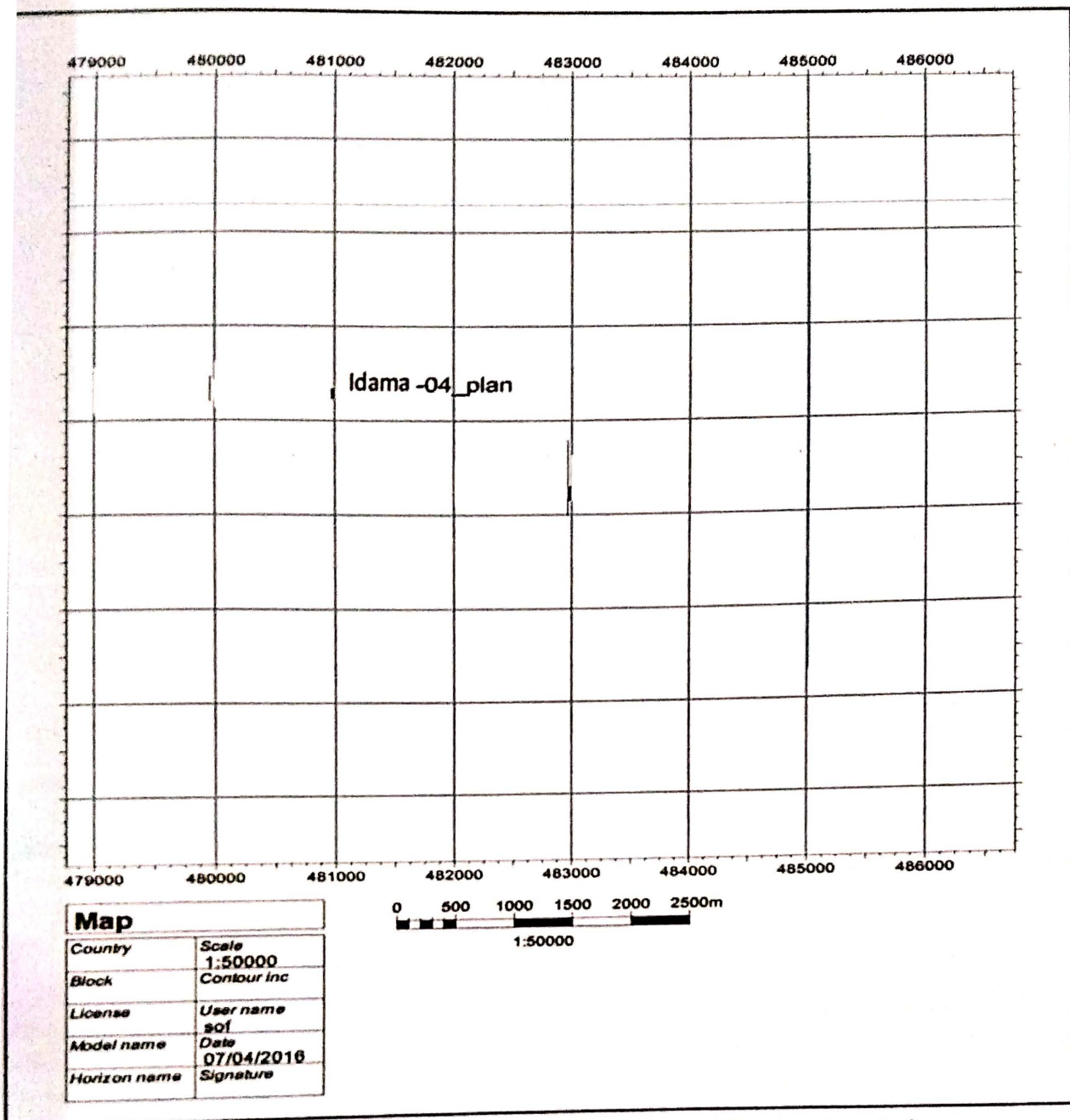
Figure 1: Base map of the study area and the locations of Ida-4 well in the Niger Delta.
