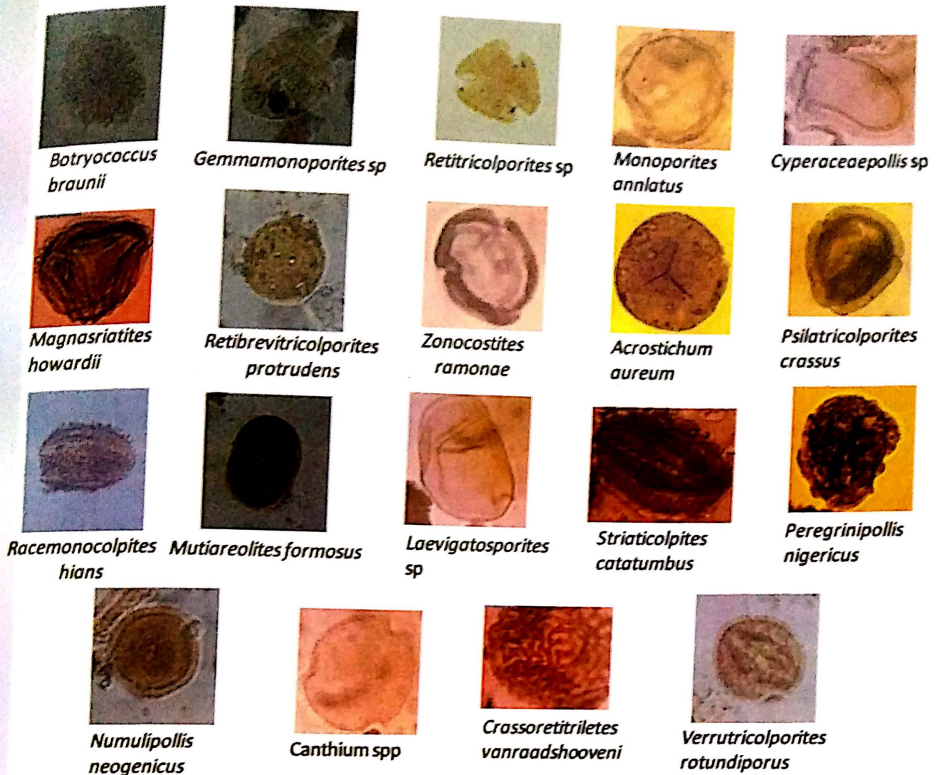
Plate 1: Palynomorphs recovered from the studied wells (x400)
