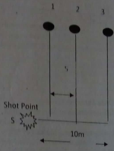
Figure 4: Field Setup of the Geophone
