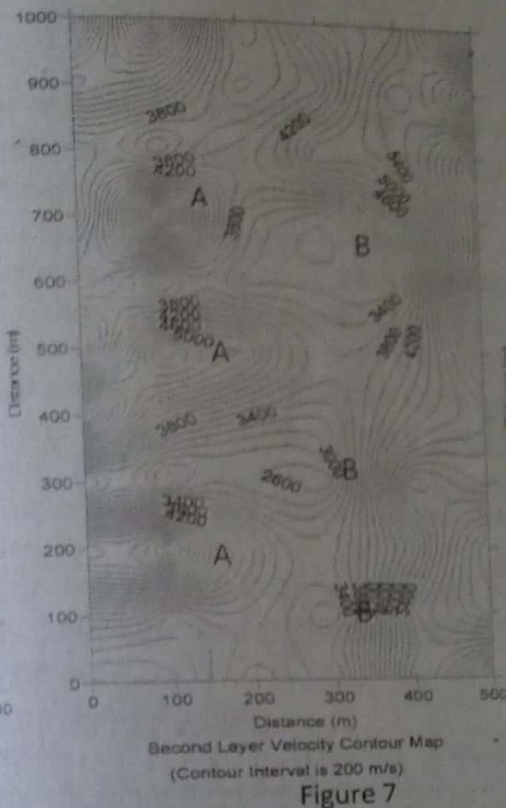
Figure 6, 7 and 8: First layer velocity, Second layer velocity and Depth to Refractor contour maps
