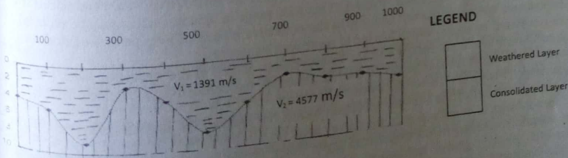
Figure 9: The geological cross section for profile B
