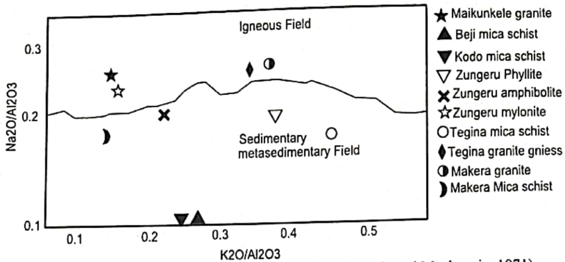
Figure 7: Na 2 O versus K 2 O plot for study area rocks (after Garrels and Mackenzie, 1971)
