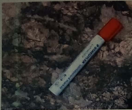
Plate I: Coarse grain granite in Gobarawa area
