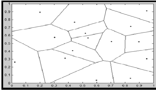
Fig 2. Voronoi diagram
