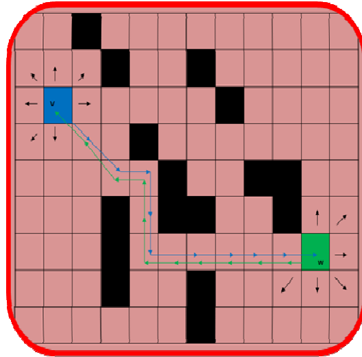
Fig 6. Bi-A* Pathfinding search process
