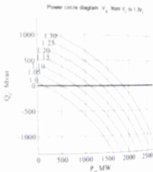
Fig. 1 Power circle diagram of tie line connecting area1 to area2
