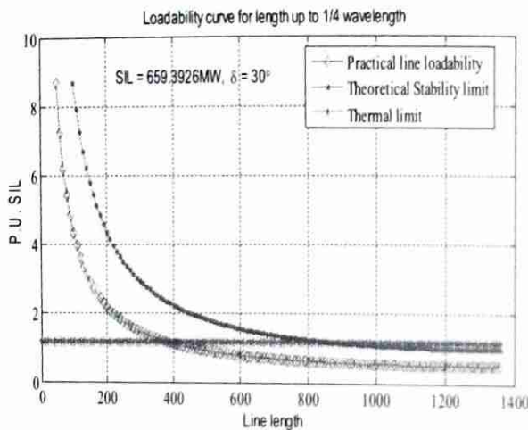
Fig. 5 Tie line load ability curve for Area 1 TO Area 2 Transfer (Jebba TS to Oshogbo)
