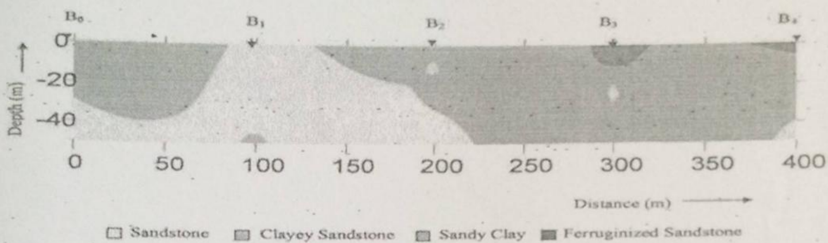
Fig. 3: Geologic Section of Profile B
