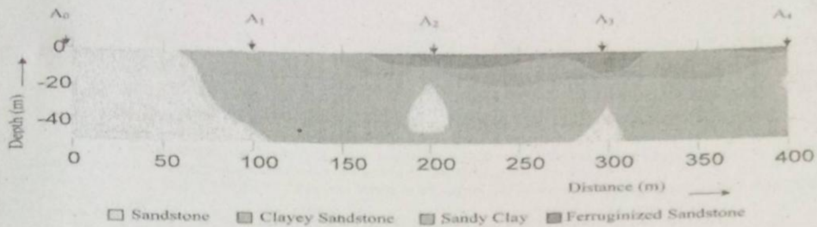
Fig. 2: Geologic Section of Profile A
