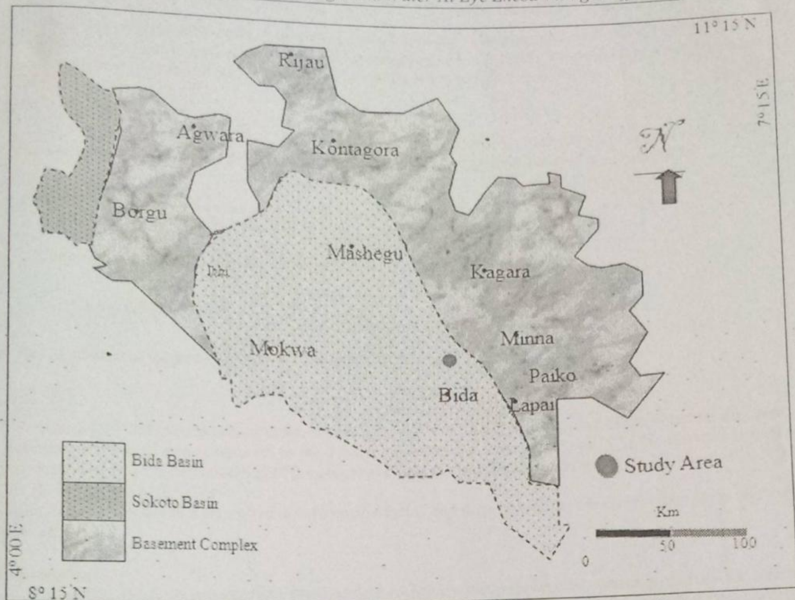
Fig 1: Geological Map of Niger State Basement Complex and Sedimentary Basins
