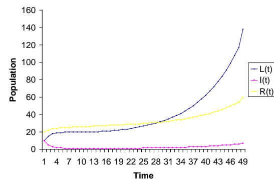
Figure 4: Closer View of L(t) , I(t) , and R(t) for \beta=0.01 and \gamma=0.23 .
