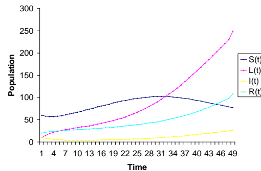
Figure 2: Graphical Profile of each Compartment for \beta=0.01 and \gamma=0.23 .
