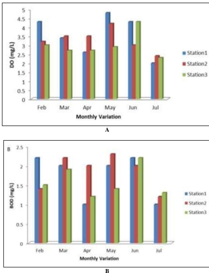
Fig 3.2: Seasonal Variations in the A) Dissolved Oxygen and B) BOD Sampled from Gurara Reservoir from Feb. to July, 2018.
