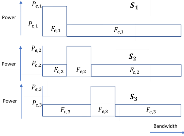
Fig. 3. Standard Downlink Resource allocation for Sectors in S_1 , S_2 and S_3
