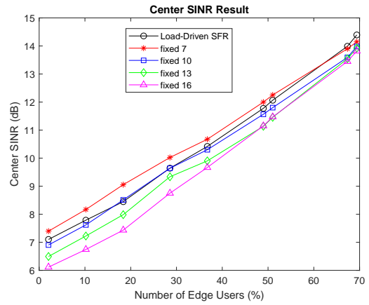
Fig. 7. Average Center User SINR performance
