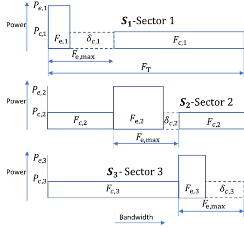
Fig. 4. Improved Downlink Resource Allocation for Sectors S_1 , S_2 and S_3
