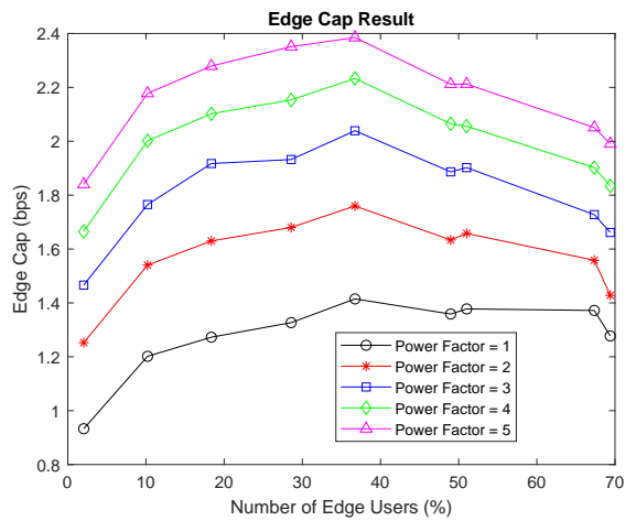
Fig. 9. Impact of Power ratio on Average Edge Capacity performance
