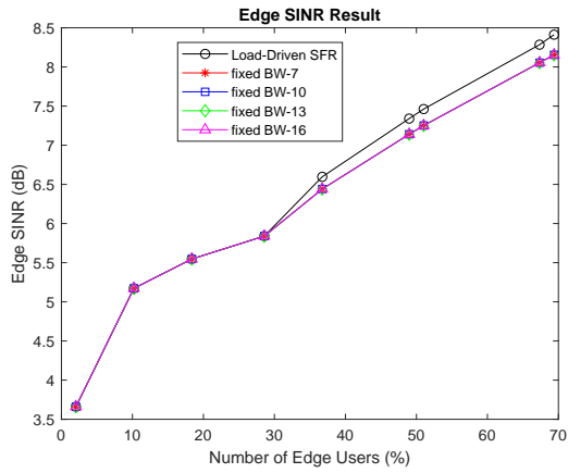
Fig. 5. Average Edge User SINR performance
