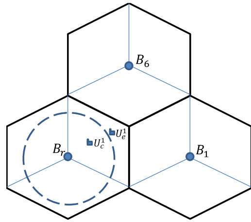
Fig. 2. Soft Frequency Reuse for three sectors including a Reference sector in B_r
