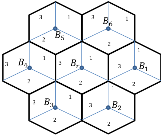
Fig. 1. Typical cellular network depicting base stations
