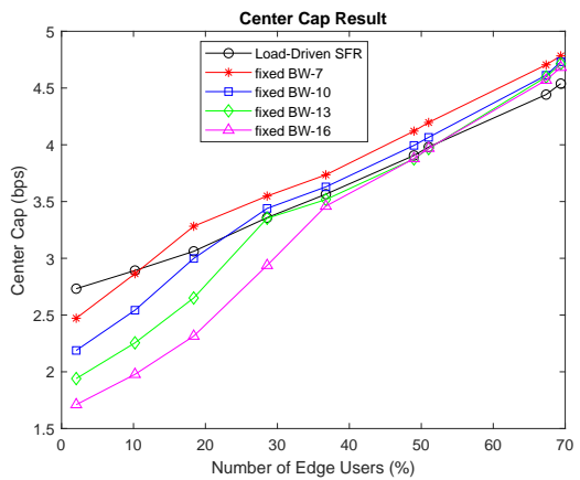
Fig. 8. Average Center User Capacity performance
