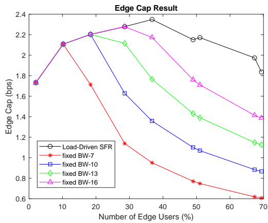
Fig. 6. Average Edge User Capacity performance
