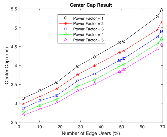
Fig. 10. Impact of Power ratio on Average Center Capacity performance
