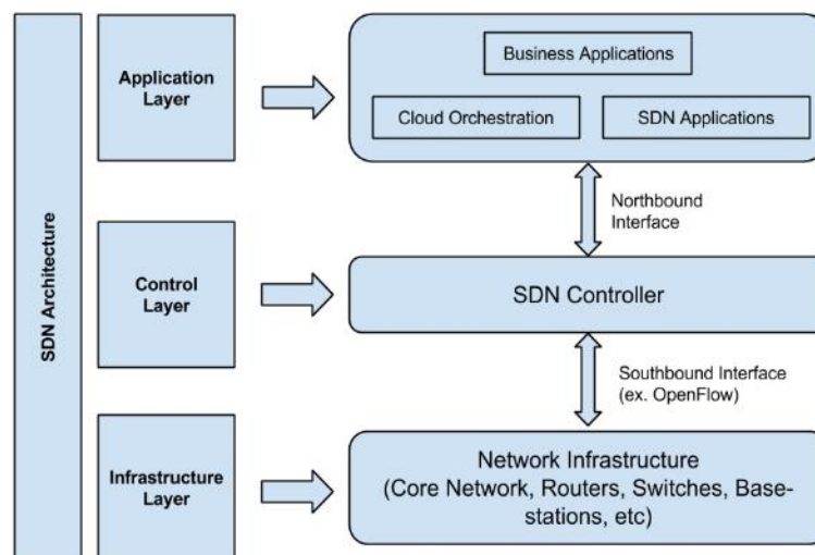
Figure 2. SDN architecture
