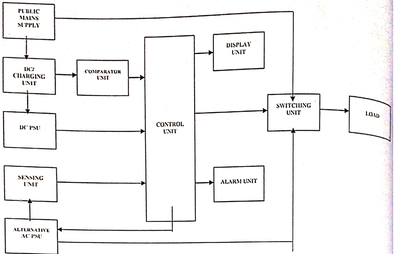
Figure 1: Block diagram of Microcontroller-based Automatic Switching System (MASS)
