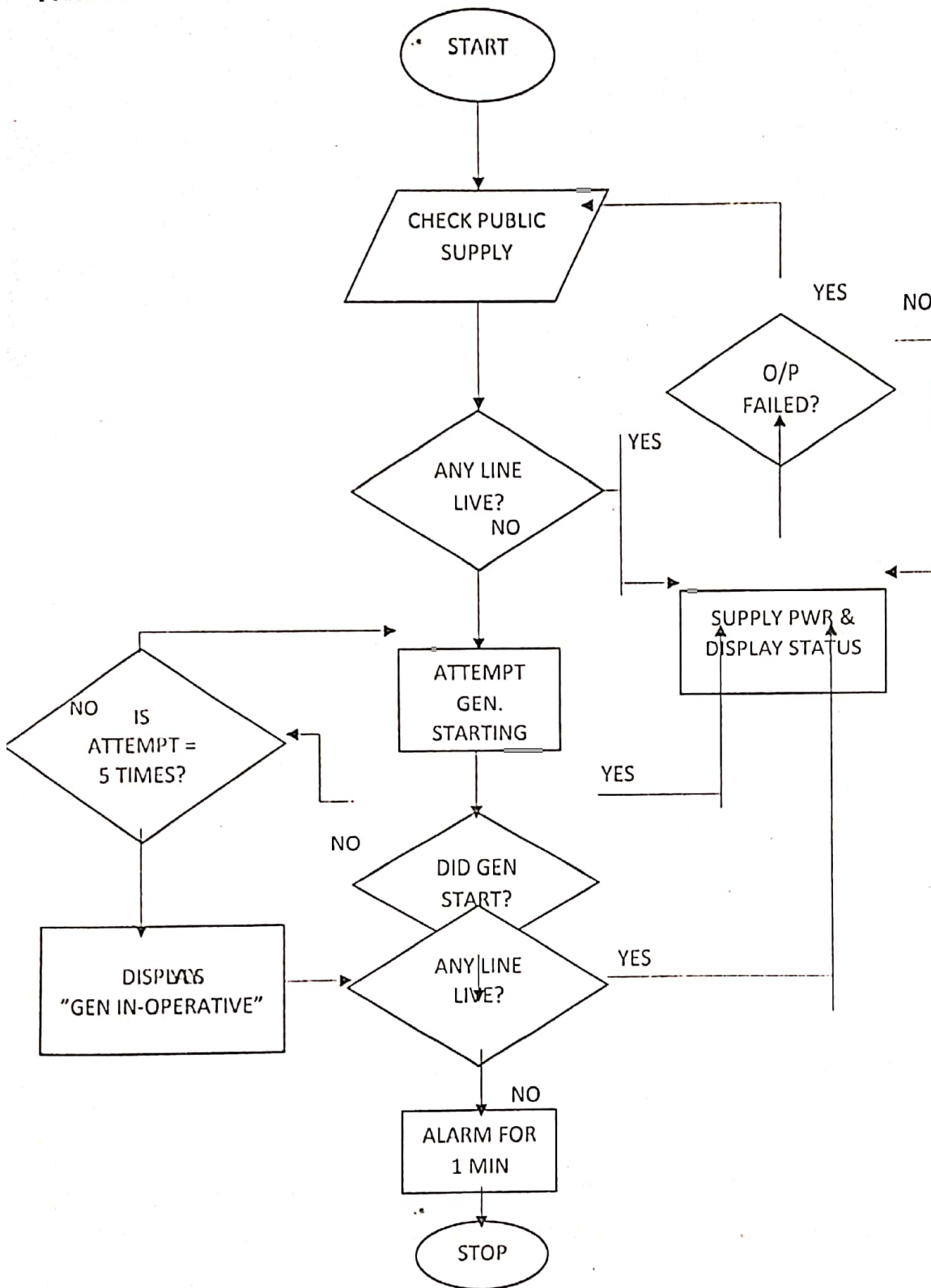
Figure 3: Flow chart of Microcontroller-based Automatic Switching System (MASS)
