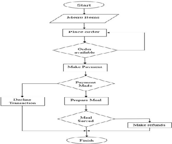
Figure 6: Flow chat of the Eatery system
