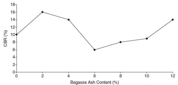
Fig. 5 Variation of California bearing ratio with bagasse ash content [16]
