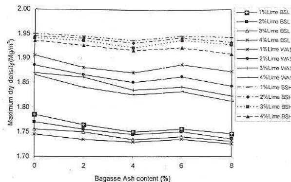
Fig. 8 Variation of maximum dry density with bagasse ash content for the different compaction energy levels [13]
