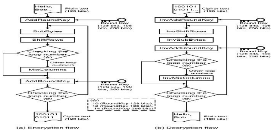
Figure 6: Process flow diagram of AES algorithm (Kumaki, Fujita, Nakanishi, & Ogura, 2013)
