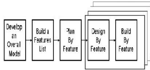
Figure 5: Feature Driven Development Approach Scheme (Palmer & Felsing, 2002)
