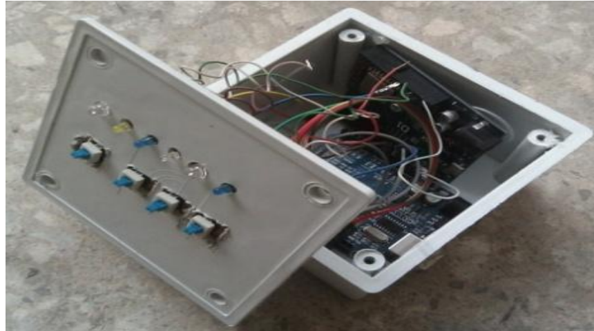
Figure 17: Developed Wireless RFID Reader
