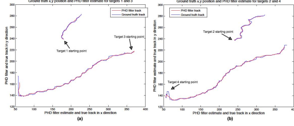
Figure 4. MTT: SMC PHD filter tracking trajectory of all 4 targets.
