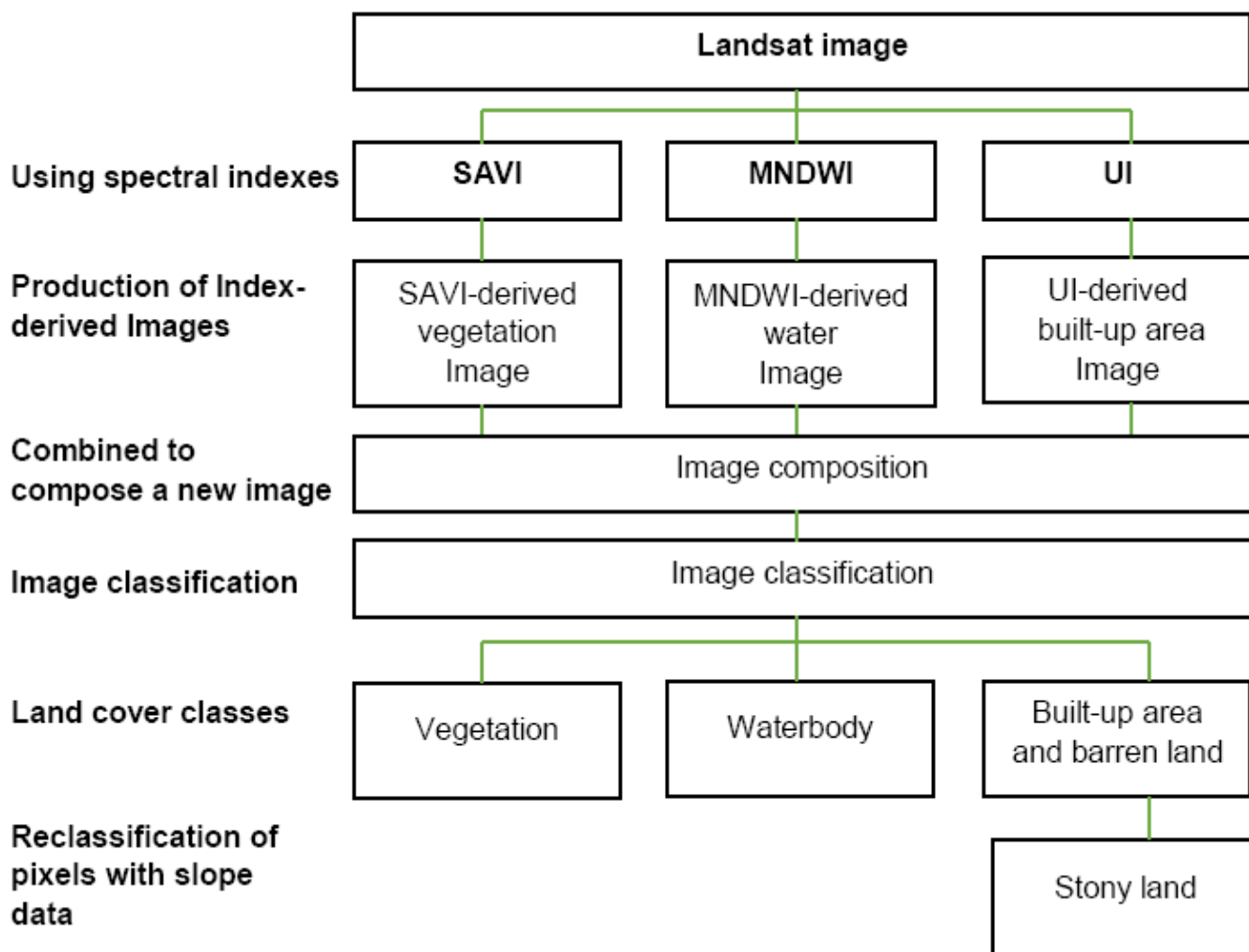
Figure 1. A classification scheme for land cover mapping (Yuan et al. , 2005).
