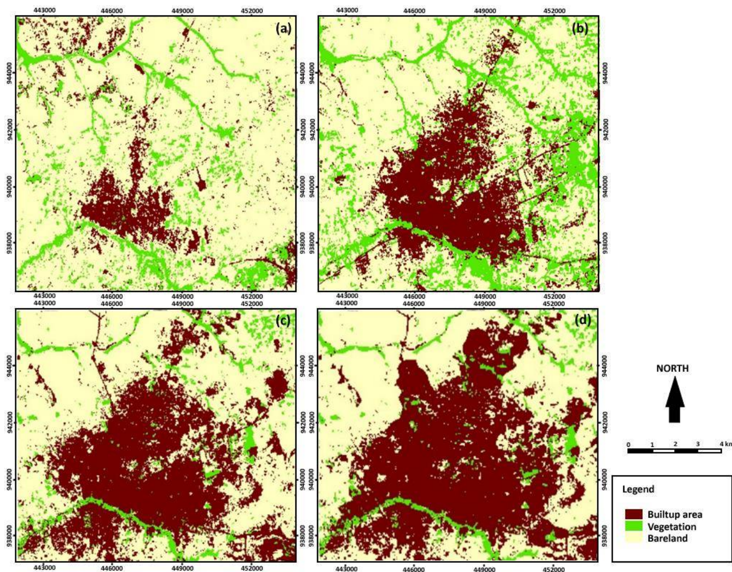
Figure 3. Spatial Extent of Lafia City. (a) Spatial extent in 1999; (b) spatial extent in 2009; (c) spatial extent in 2019, and (d) spatial extent 2029 based on simulation.
